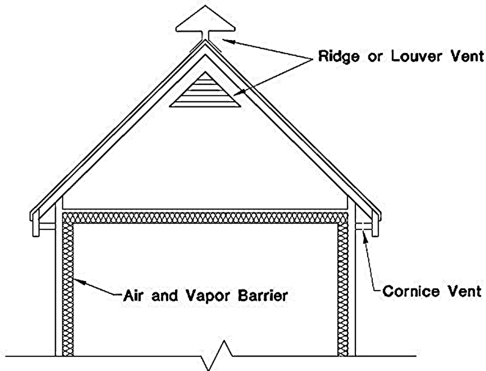
Vented Attic Space
