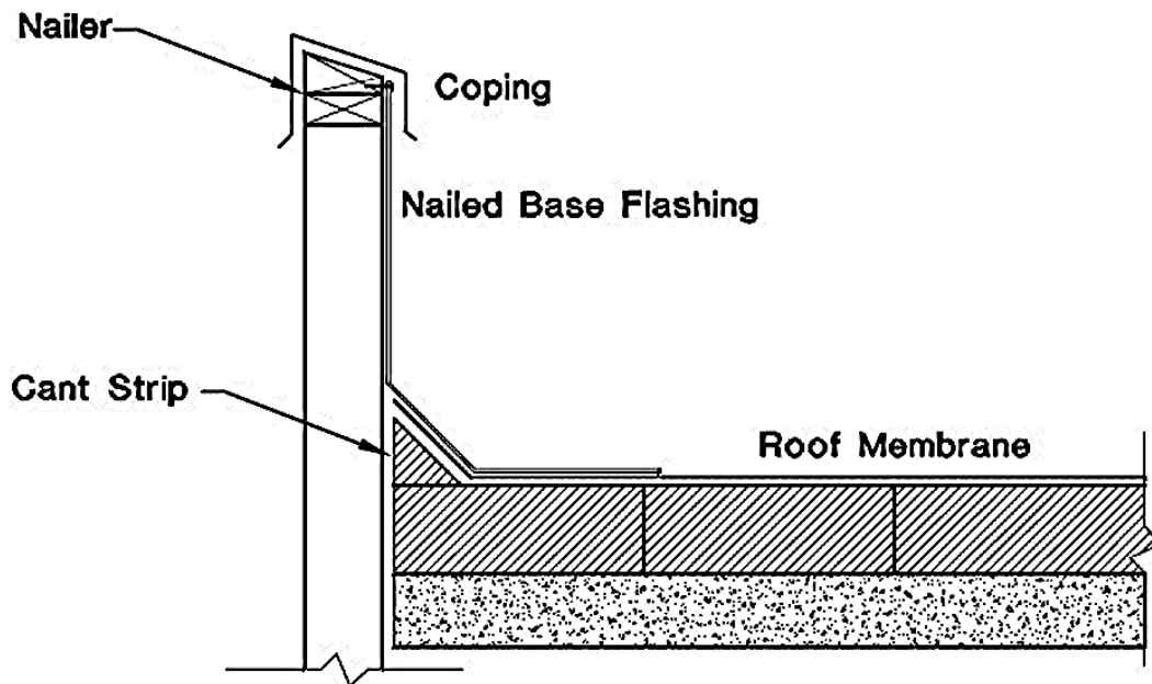
Wall Base and Cap Flashing
