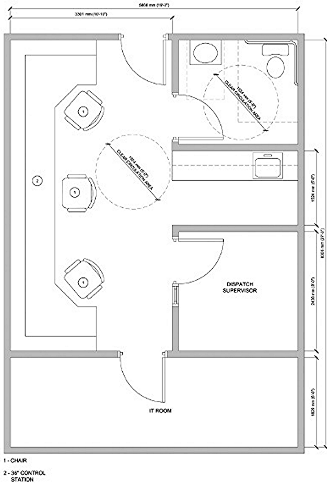
Figure 2-14 Larger Dispatch Room
