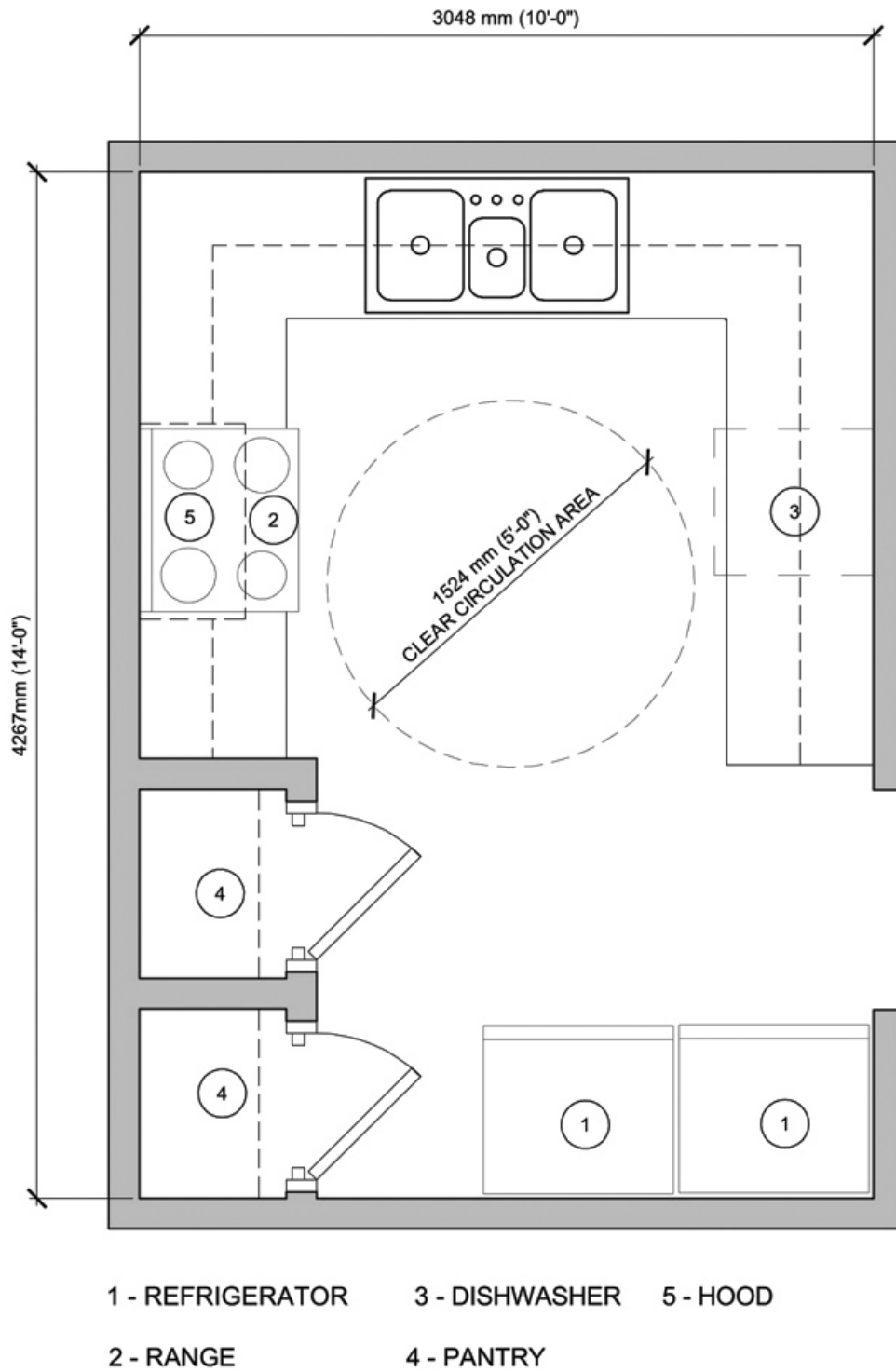
Figure 2-16 Day Room - Kitchen
