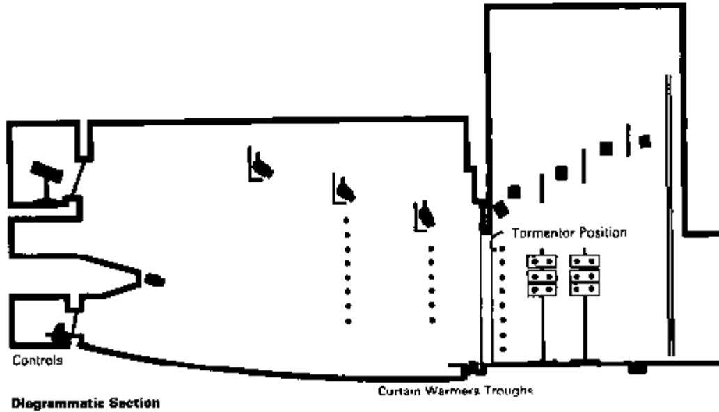
Figure 39 Lighting positions
