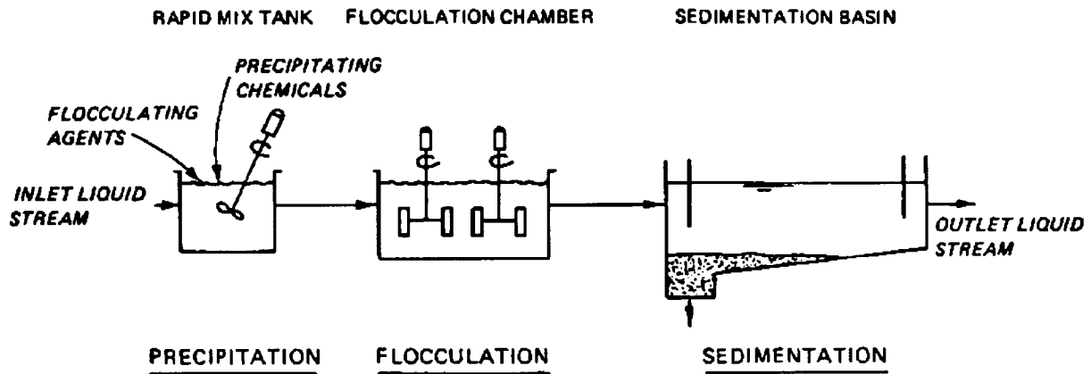
Figure 4-13. Representative Configuration Employing Precipitation, Flocculation, and Sedimentation
