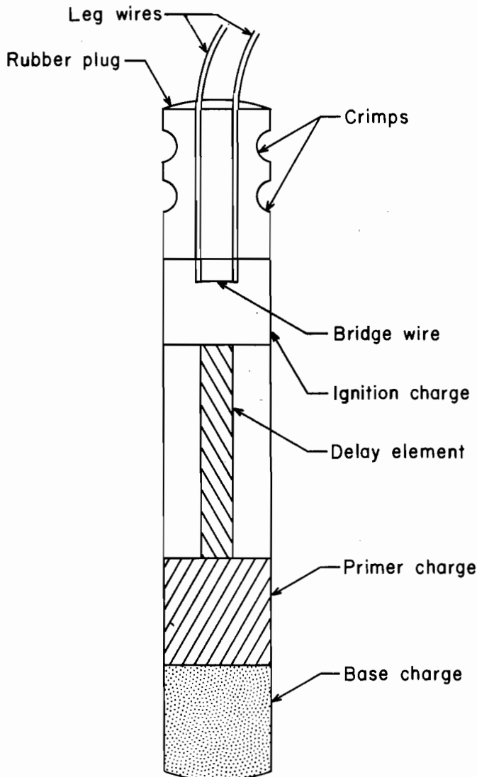
Figure 20.—Delay electric blasting cap.
