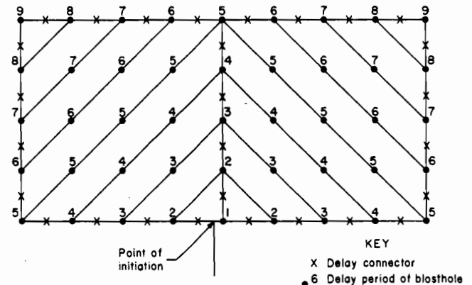
Figure 33.—Typical blast pattern with surface delay connectors.
