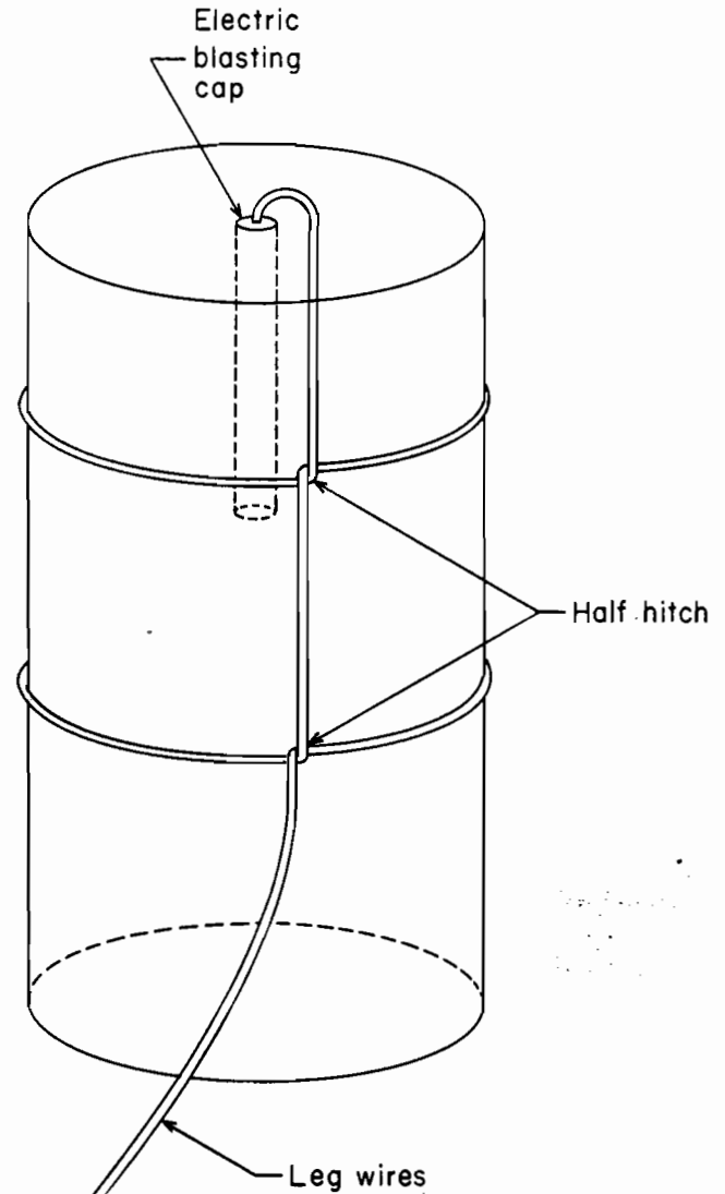
Figure 49.—Cartridge primed with electric blasting cap.
