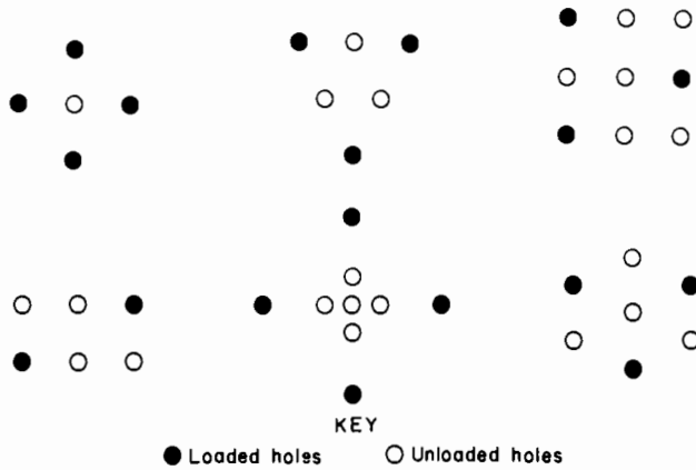
Figure 77.—Six designs for parallel hole cuts.
