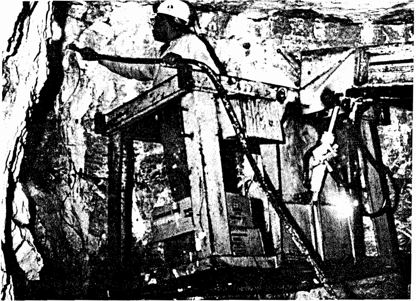
Figure 53.—Pneumatic loading of AN-FO underground. (Courtesy Hercules Inc.)
