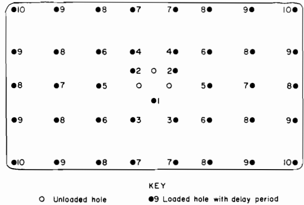
Figure 85.—Typical burn cut blast round delay pattern.
