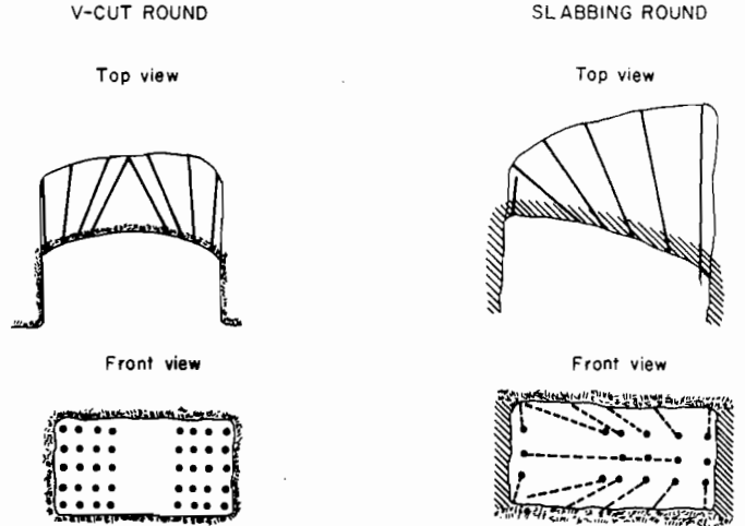
Figure 81.—Angled cut blast rounds.
