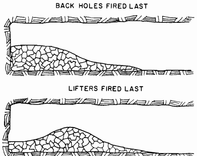
Figure 87.—Shape of muckpile as a function of order of firing.
