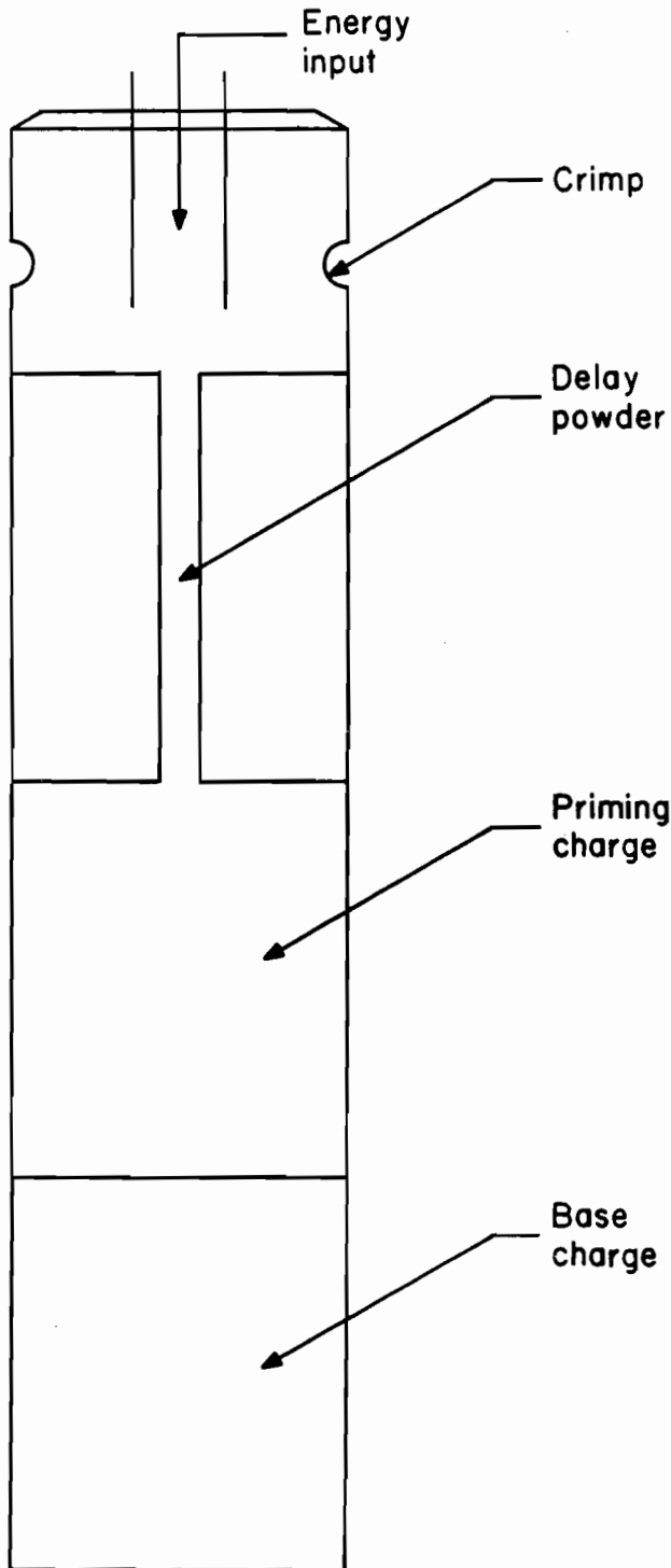
Figure 18.—Delay detonator.
