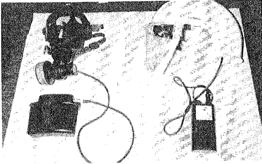
Pictured above are two different types of powered air-purifying respirators (PAPR's) equipped with high-efficiency filters. On the left is an example of a tight fitting, full facepiece PAPR, and on the right is an example of a loose-fitting helmet style PAPR.
