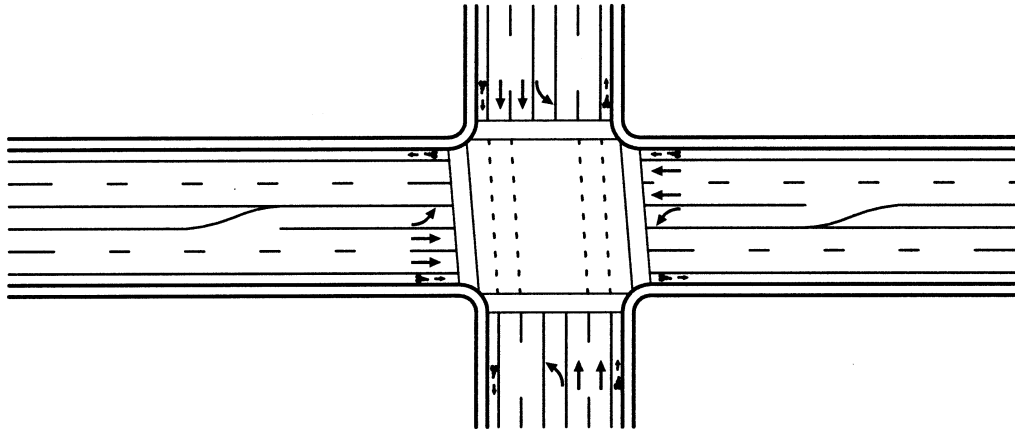
Figure 121. Example of delineated paths.
