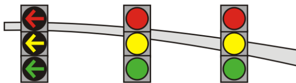
(a) Protected left-turn phasing using a three-section signal head with red, yellow, and green arrows.
