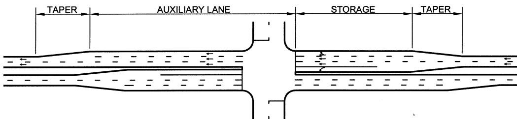
Figure 120. Diagram of an auxiliary through lane. (adapted from 199)
