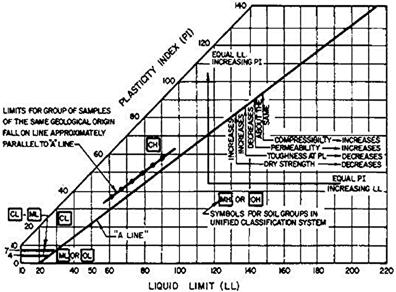
Figure 2 Utilization of Atterberg Plasticity Limits
