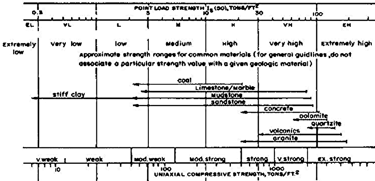
Figure 3 Strength Classification
