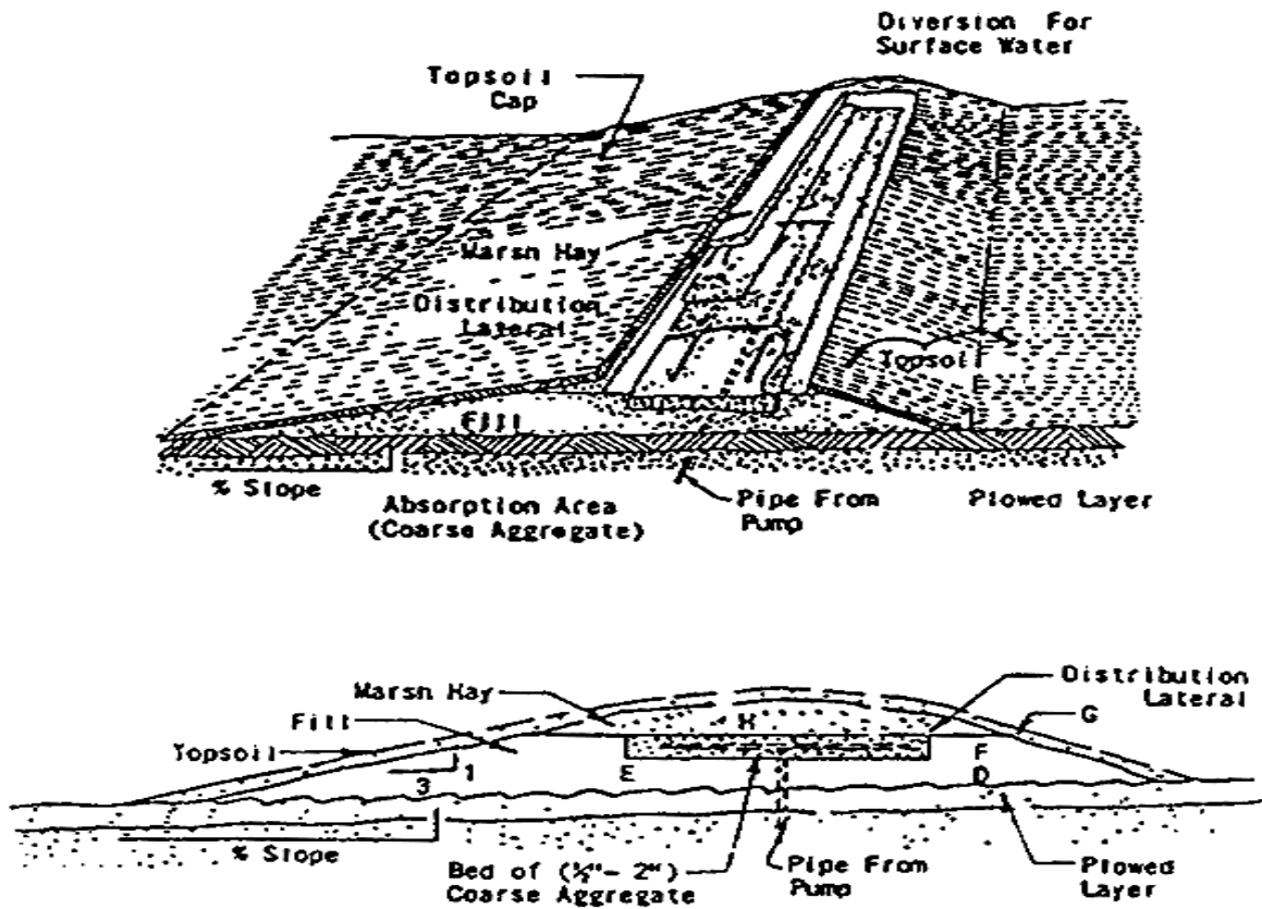
A detailed cross-section of a mound using a bed for the absorption area. Normally used on shallow permeable soils with creviced bedrock or permeable soils with high water tables.
