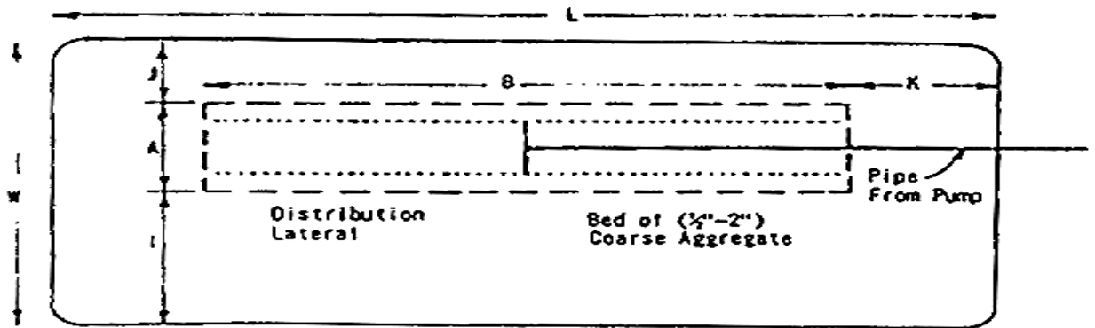
A detailed plan view of a mound using a bed for the absorption area.
