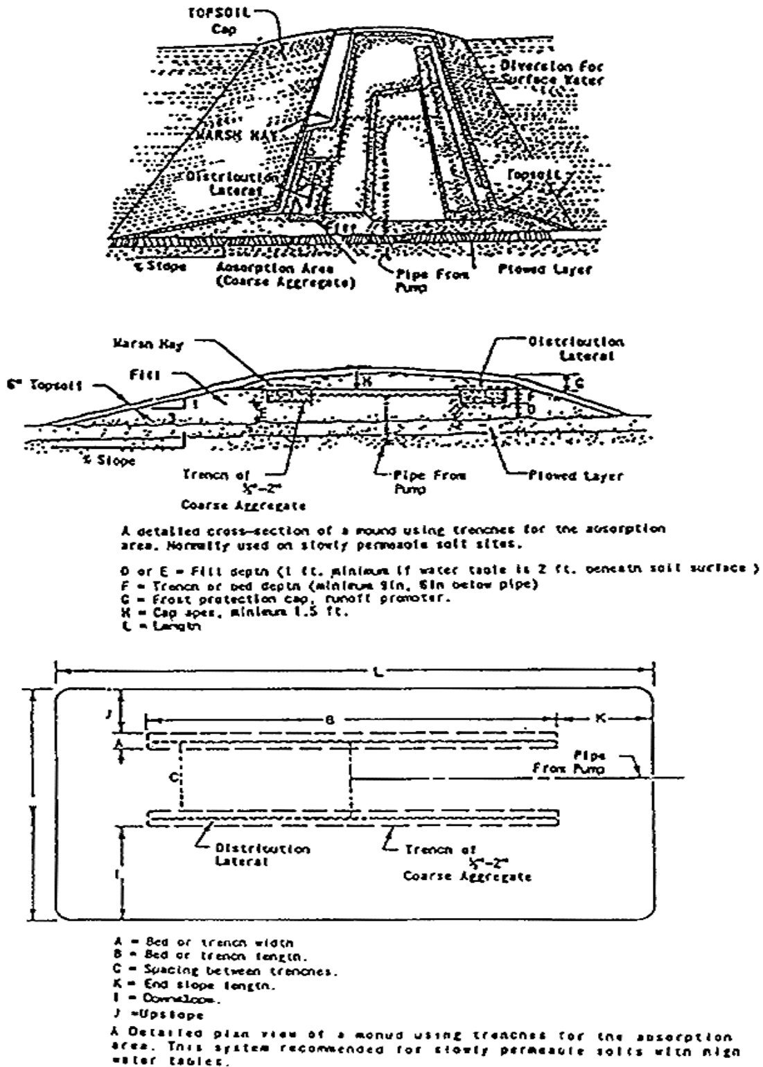
Figure 5-1 Mound system - trenches
