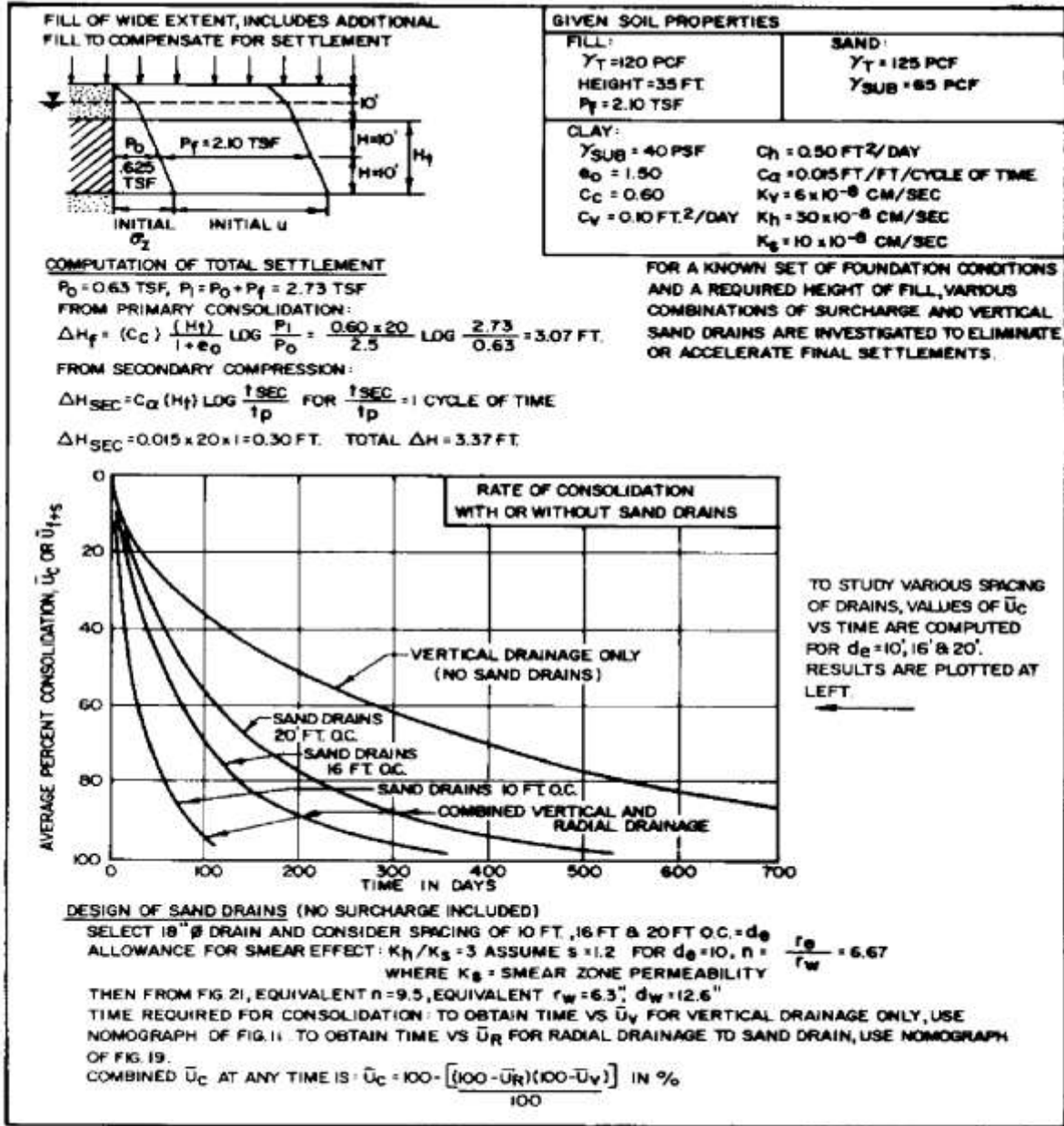
FIGURE 20 Example of Surcharge and Sand Drain Design
