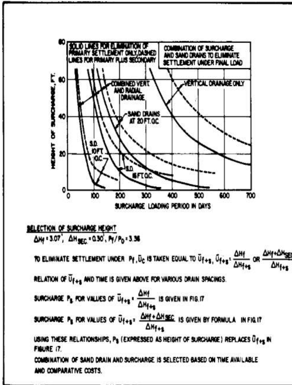
FIGURE 20 (continued) Example of Surcharge and Sand Drain Design
