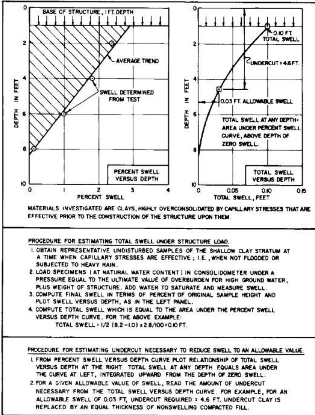
FIGURE 22 Computation of Swell of Desiccated Clays
