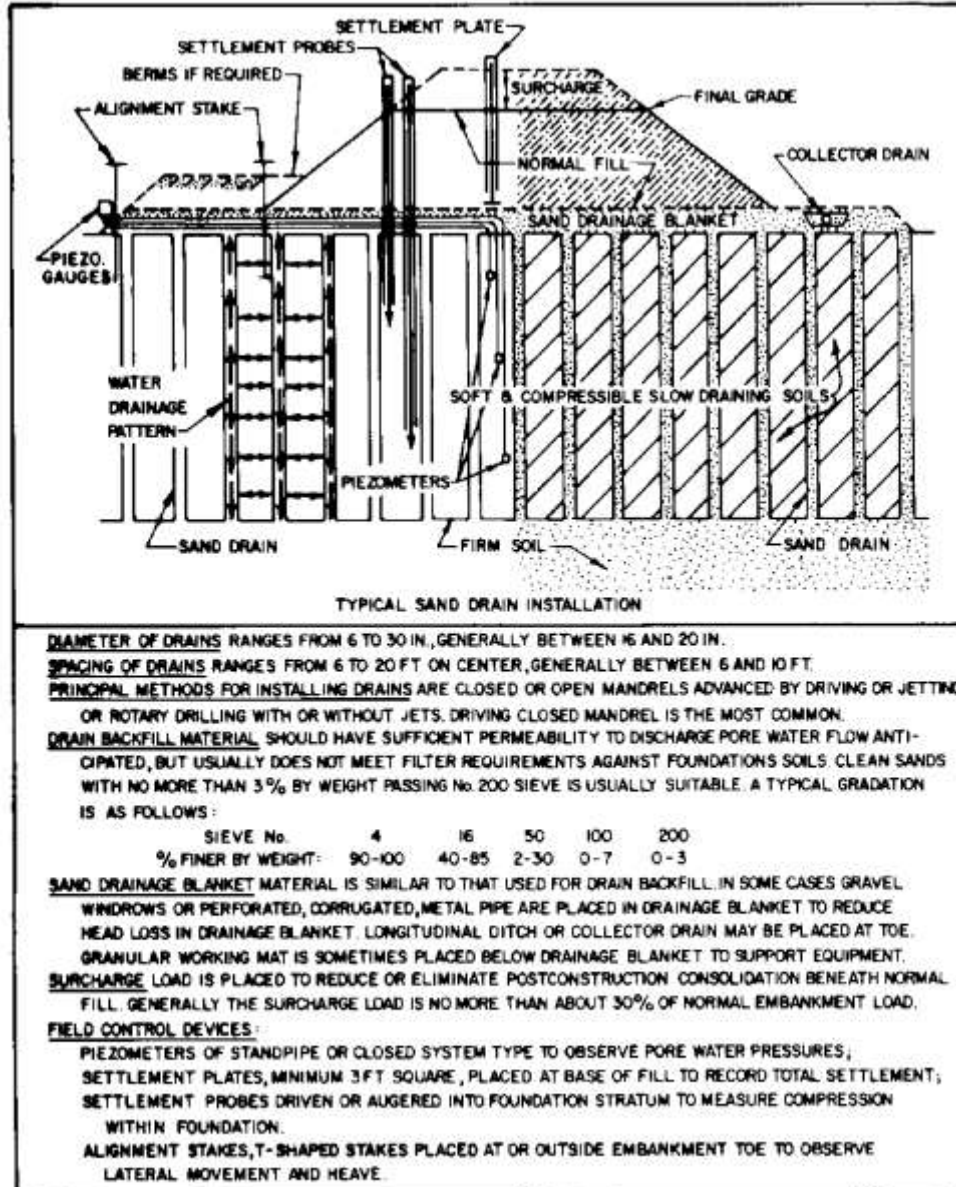
FIGURE 18 Data for Typical Sand Drain Installation
