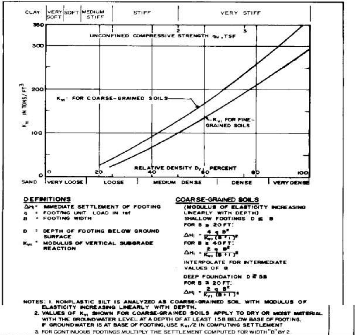
FIGURE 6 Instantaneous Settlement of Isolated Footings on Coarse-Grained Soils
