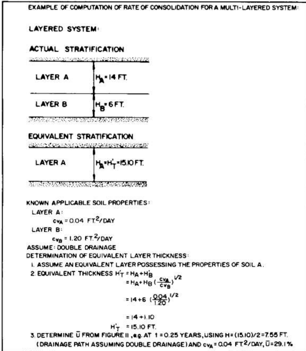
FIGURE 15 (continued) Procedure for Determining the Rate of Consolidation for All Soil Systems Containing "N" Layers
