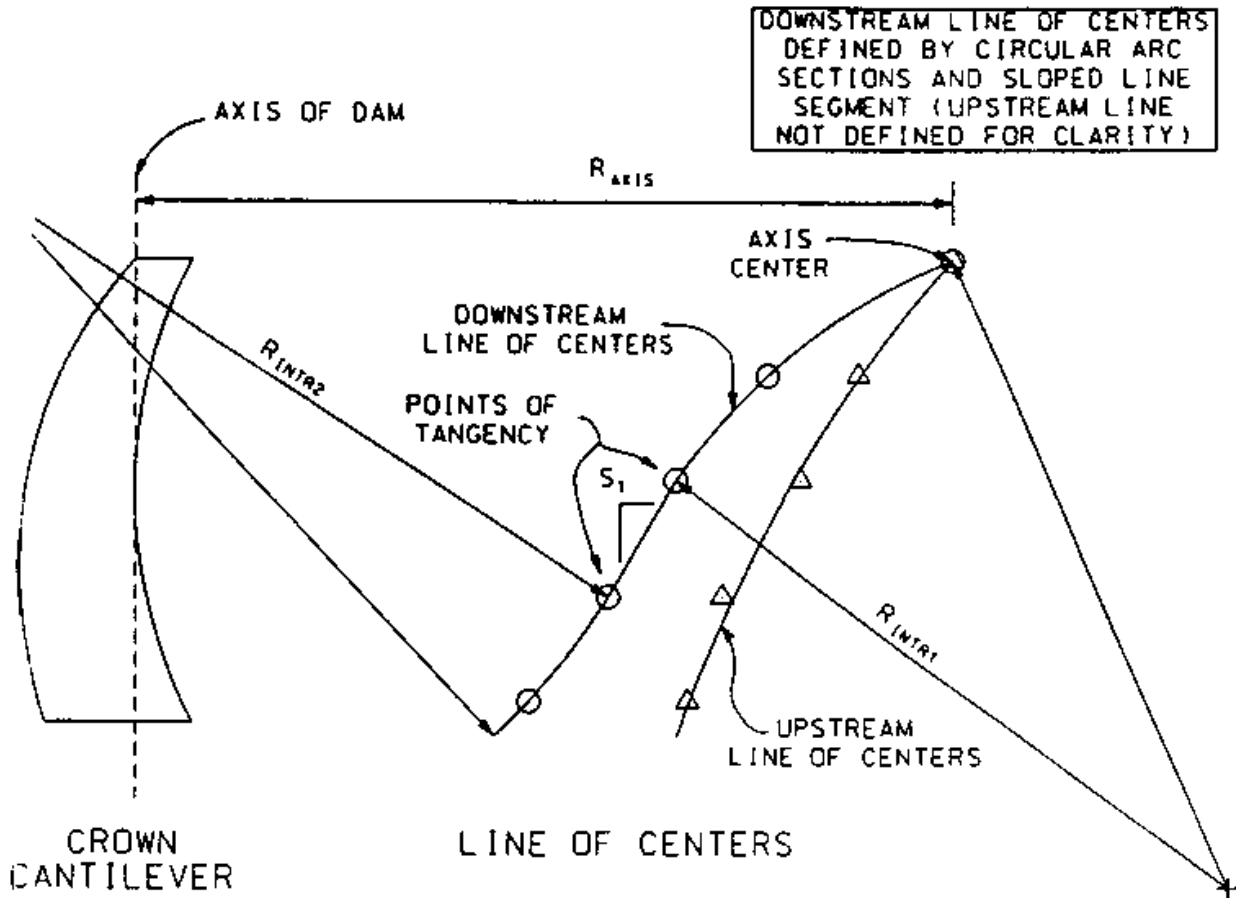
Figure 5-10 Defining the lines of centers
