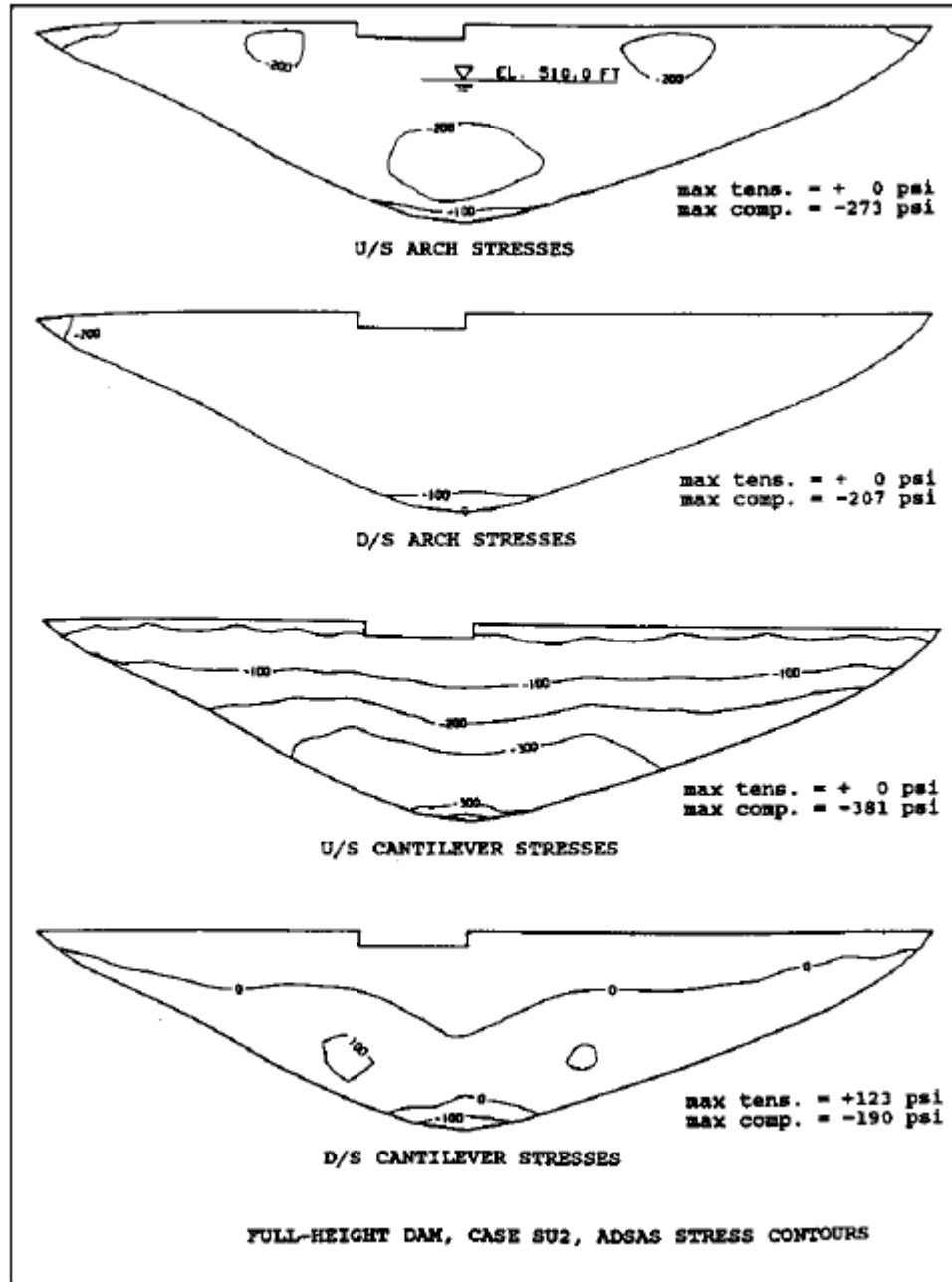
Figure 5-18 ADSAS stress contours
