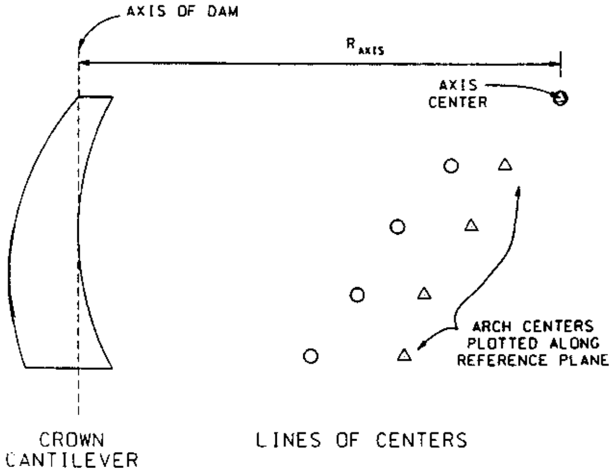
Figure 5-8 Plotting of arch centers along reference
