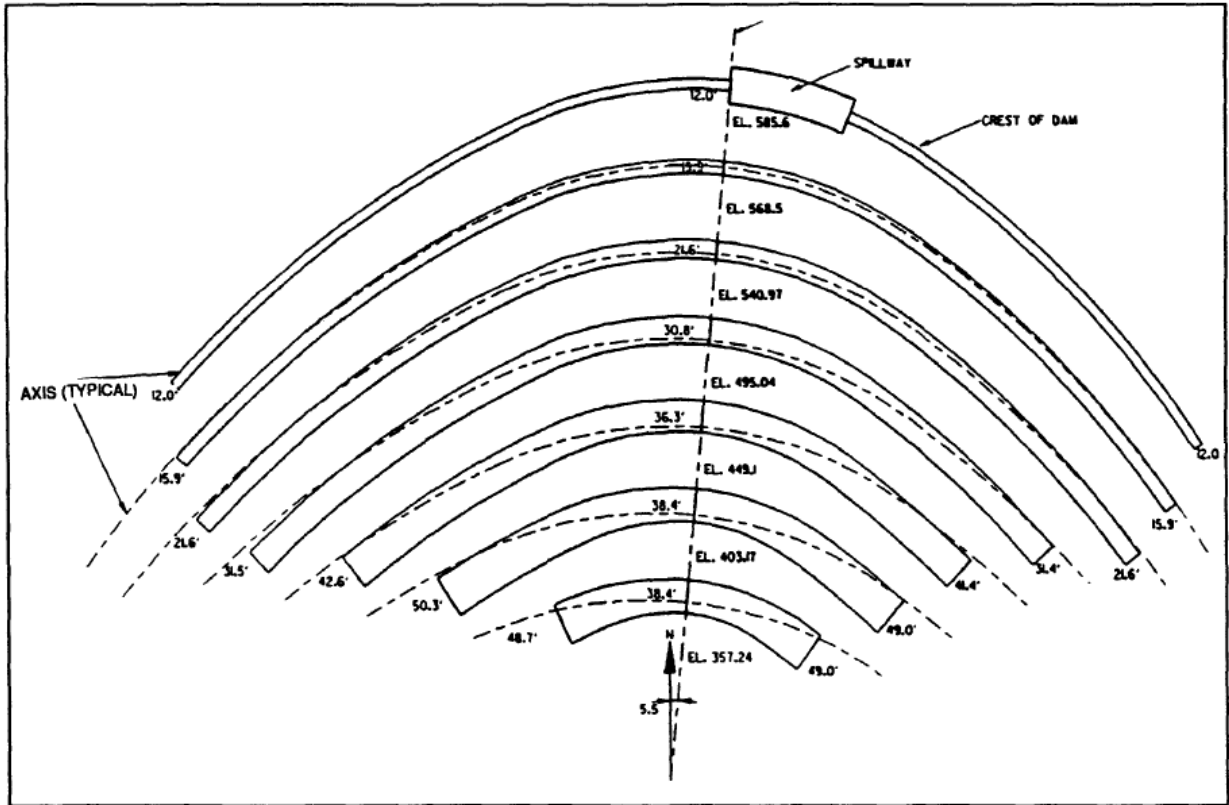
Figure 5-15. Arch sections
