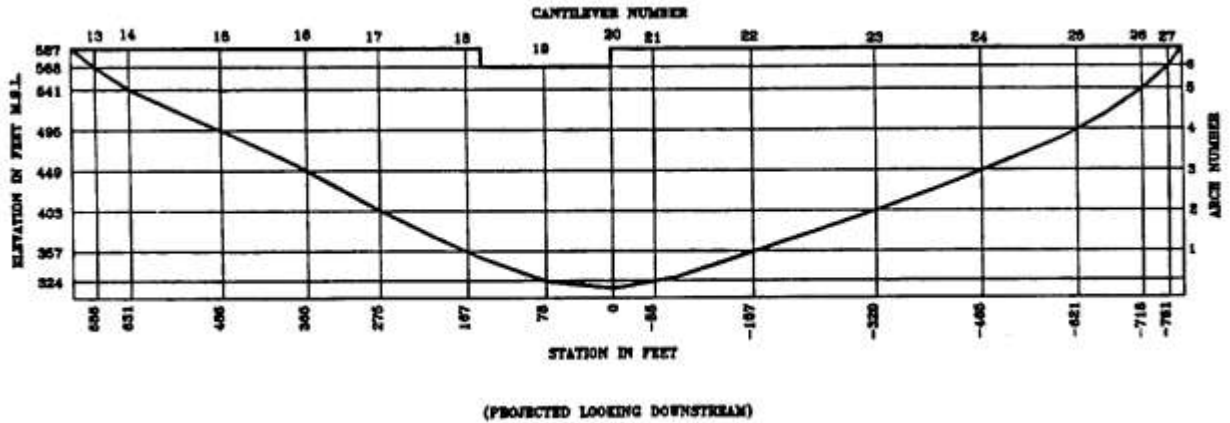
Figure 5-17 ADSAS model
