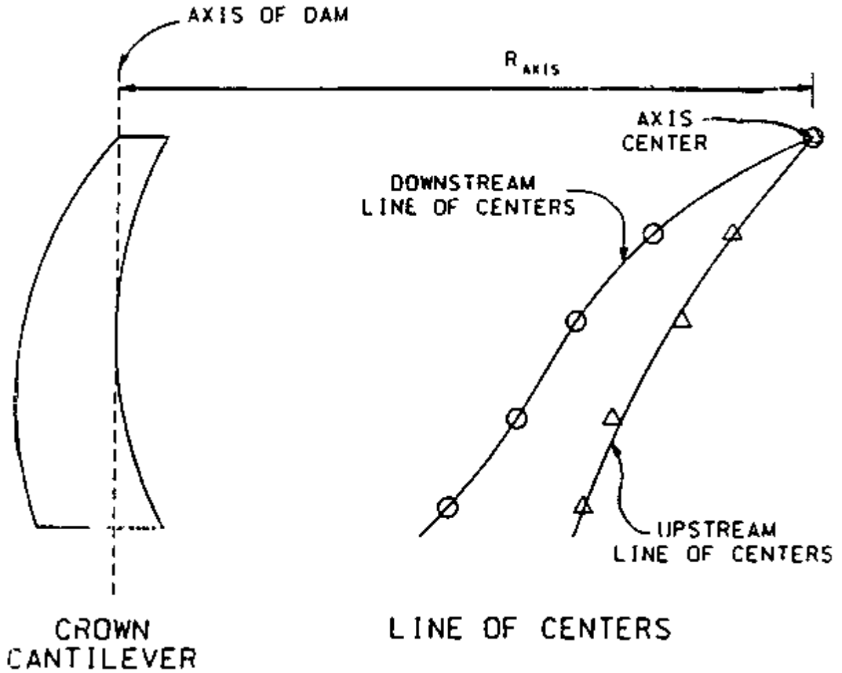
Figure 5-9 Development of the lines of centers
