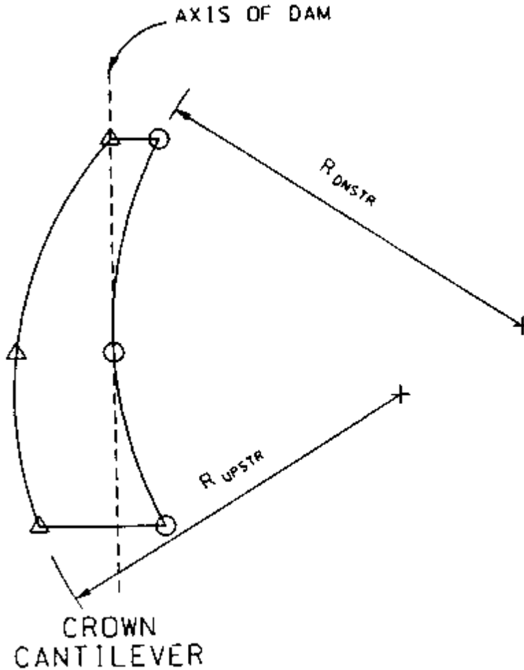
Figure 5-4 Definition of upstream and downstream faces
