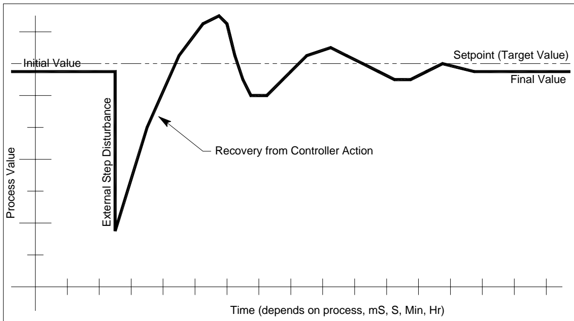
Process Trend Chart - Good Tuning, High Gain
