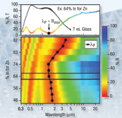
A custom software tool developed under the EM&D project facilitates the display and analysis of optical data for transparent conducting oxides, which are important components of many PV devices.
