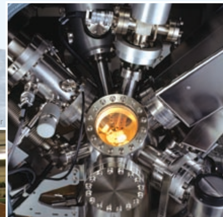
The M&C project's surface analysis cluster tool is used for studies of surface chemistry and physics using techniques such as Auger electron, X-ray photoelectron, and ultraviolet photoelectron spectroscopies, and thermal desorption mass spectrometry.
