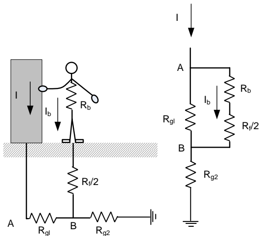
Figure 9. Touch potential
