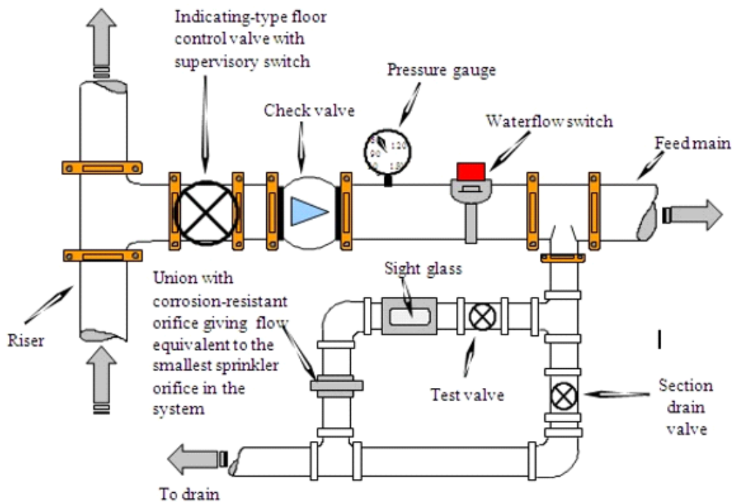
Figure 7 Floor Control Valve Assembly
