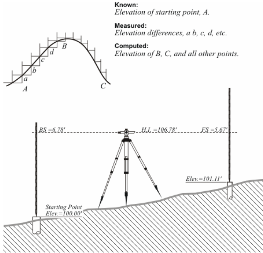
Figure 3.4 Spirit leveling.
