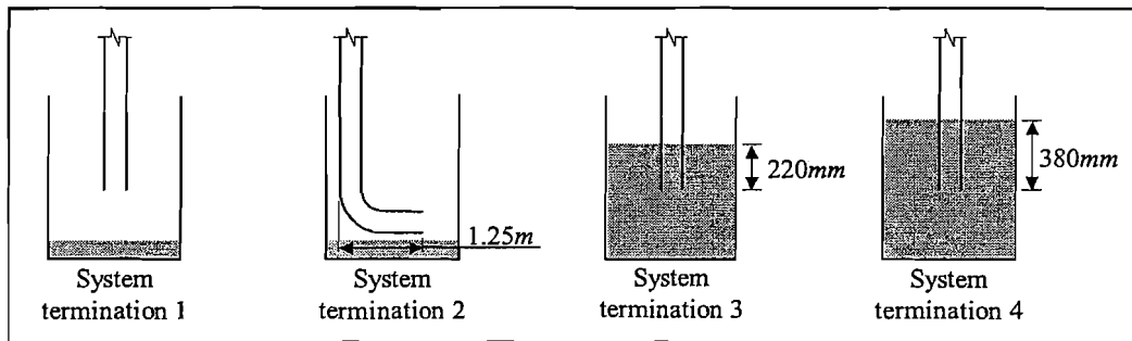
Figure 7: Siphonic system termination configurations investigated
