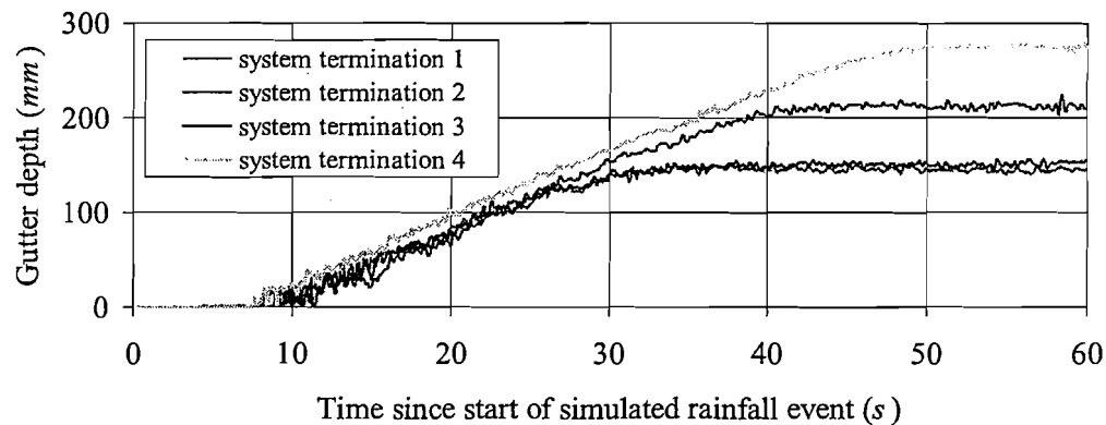
Figure 8b: Variation in gutter I flow depth (T1) with system termination configuration (fully primed conditions)
