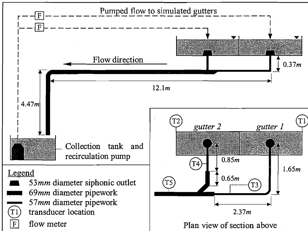
Figure 2: Siphonic roof drainage experimental test rig
