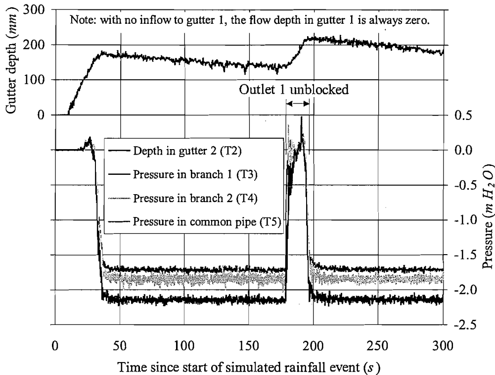
Figure 6: Measured gutter depths and system pressures with the outlet in gutter 1 blocked/unblocked/blocked ( gutter 1 inflow = 0l/s, gutter 2 inflow = 11.3l/s)
