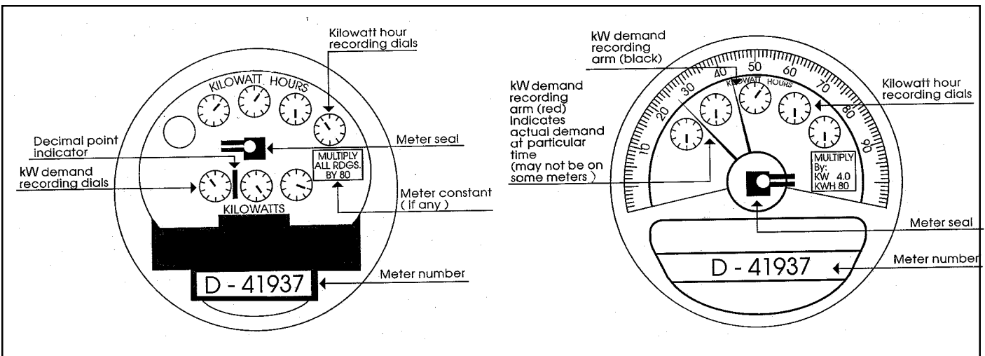
Figure 2-4 Electric Demand Meters
