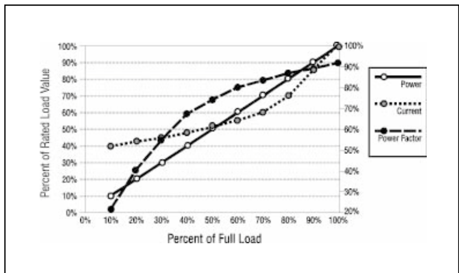
Figure 5-1 Relationships Between Power, Current, Power Factor and Motor Load
