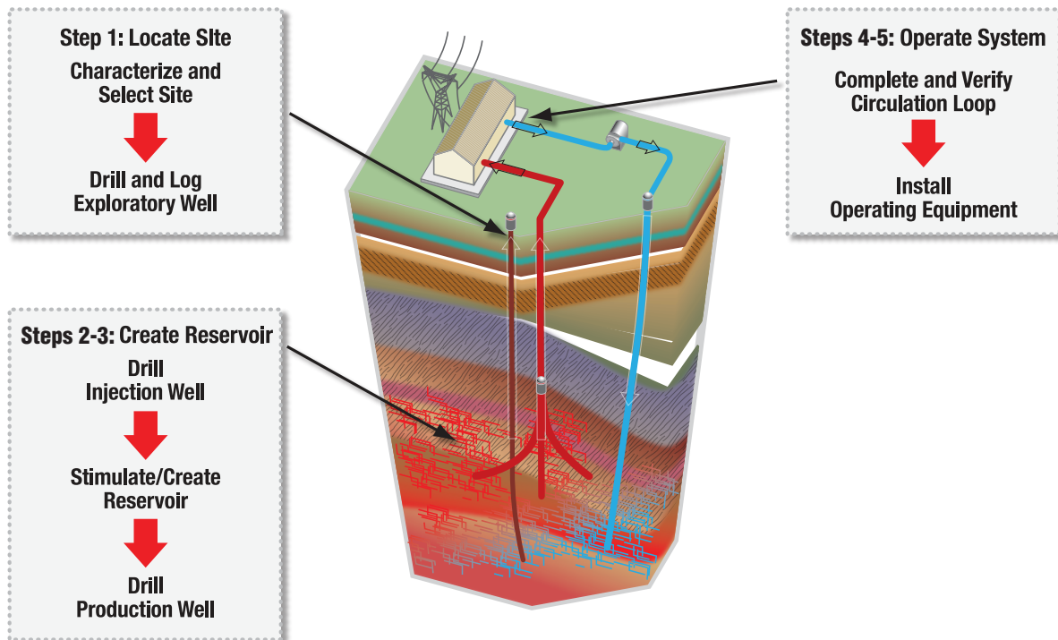
Figure 3. EGS Development Sequence
