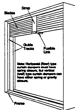
Figure 2. Curtain Fire Damper [adapted from SMACNA (1986)].
