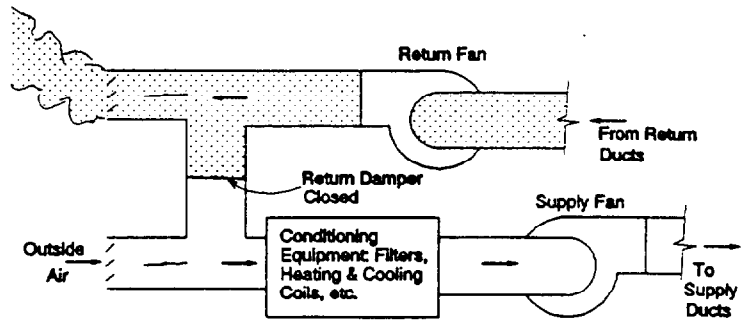
Figure 5. HVAC System With Recirculation Capability in the Smoke Control Mode.
