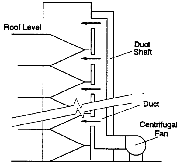
Figure 6. Stairwell Pressurization by Multiple Injection With the Fan Located at Ground Level.
