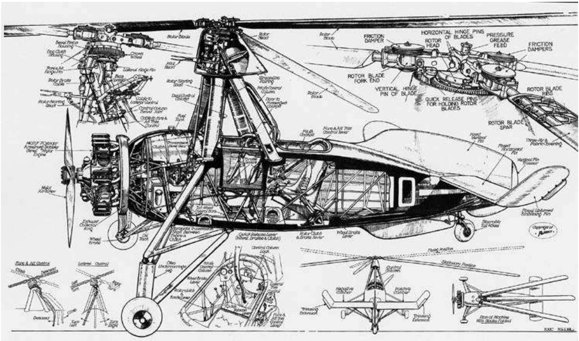
Above: caption: “Cierva C.30A. The Cierva was a practical non-stalling production Autogyro with cantilever rotor and reliable shaft and clutch for direct engine-to-rotor starting. About 70 C.30s were built under license by A.V. Roe, and a further 75 were produced in France and Germany. An example is kept in the Science Museum, London.”
