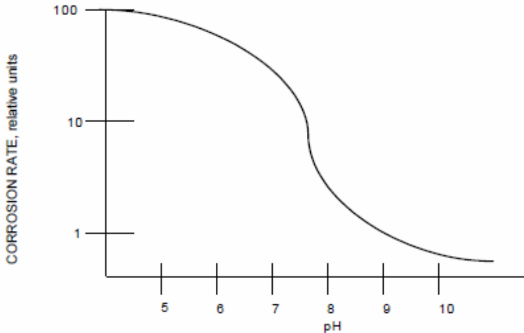
Figure 19 Effect of pH on corrosion rate of unprotected mild steel in water
