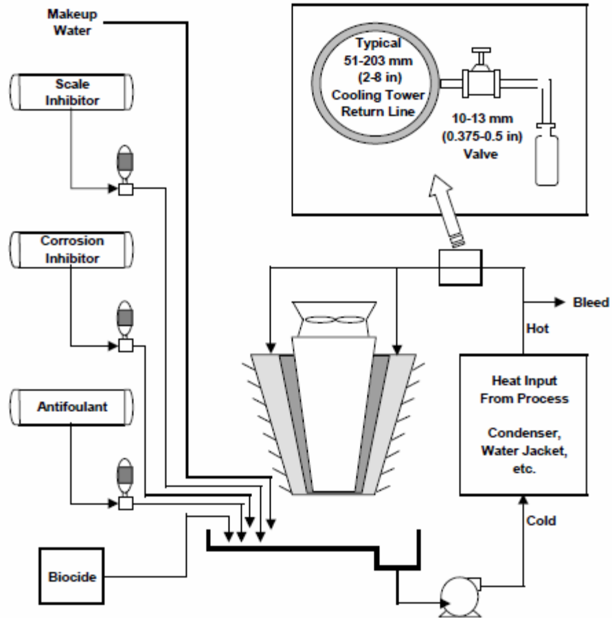
Figure 1 Typical Water Sampling Points for an Open Recirculating Cooling Water System
