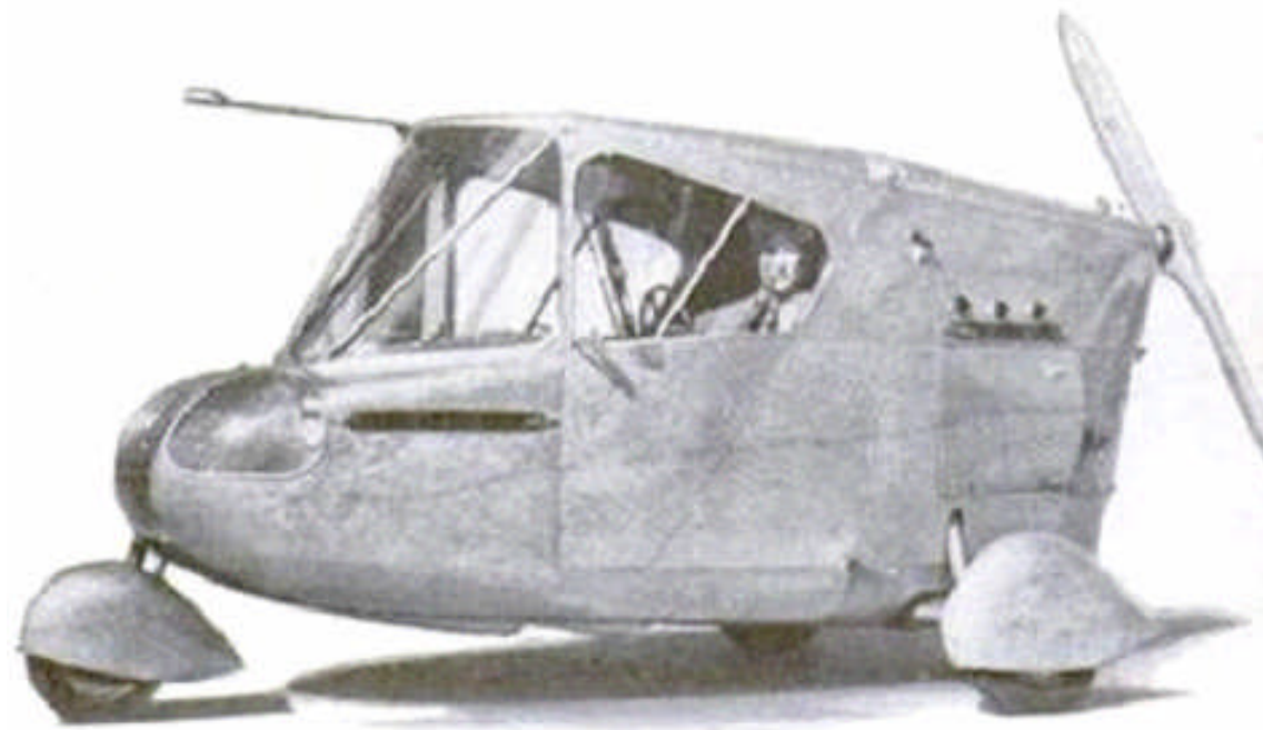
Above & Left: caption: “Detachable wings enable a vehicle of odd design to travel on the ground as well as in the air. Capable of attaining a speed of 110 mph while flying and 55 on the ground, the novel craft is powered by a standard six-cylinder automobile engine. Above, the auto-plane making a landing; Left, the auto-plane with wings detached for use on ground as a car”
