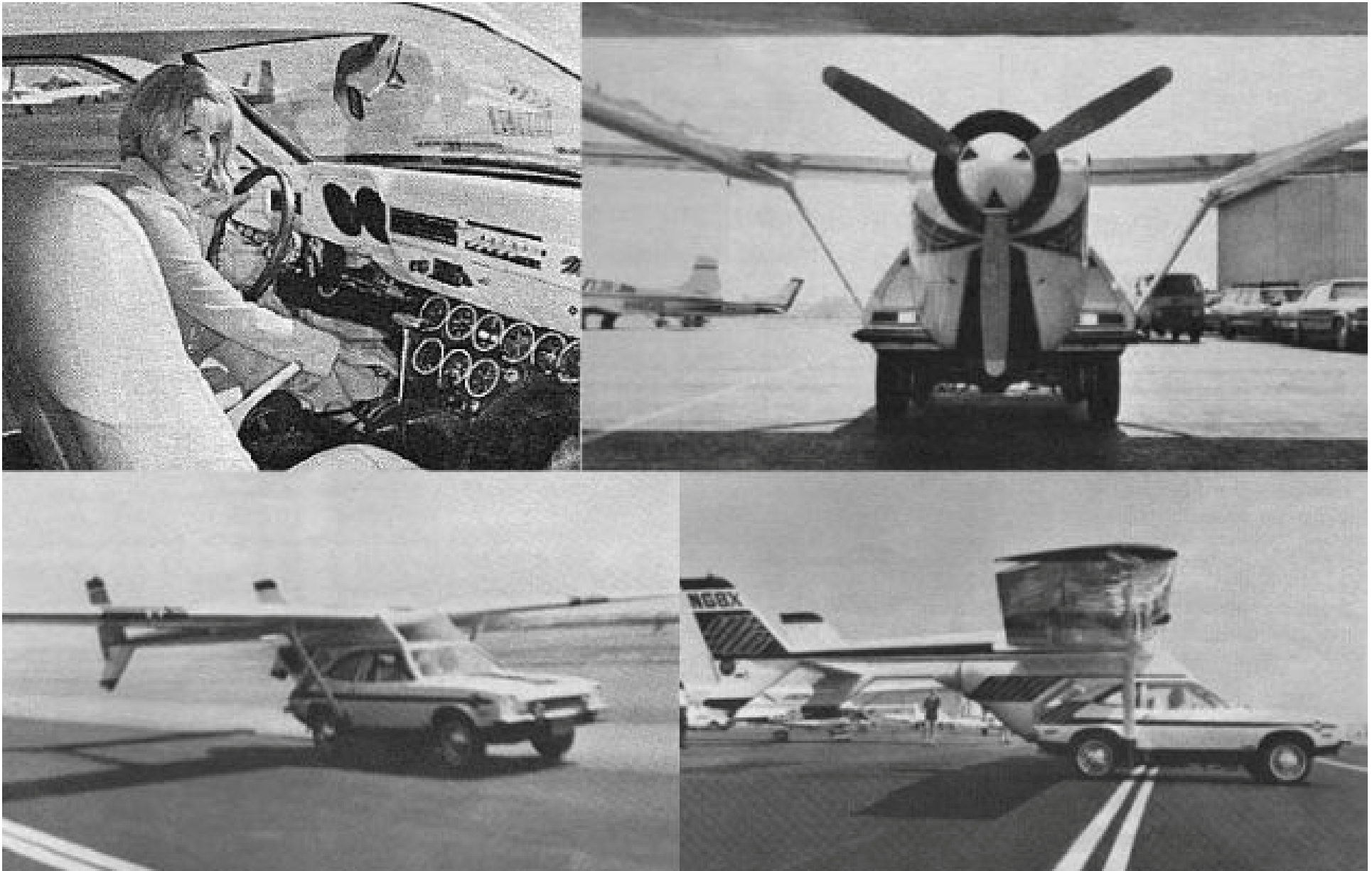
Above: caption: “The AVE Mizar, a roadable airplane. The prototype Mizar has a 210 Continental, but future models will run up to a 300-hp Lycoming. The Pinto’s dash has altimeter, airspeed indicator and other flight instruments.
