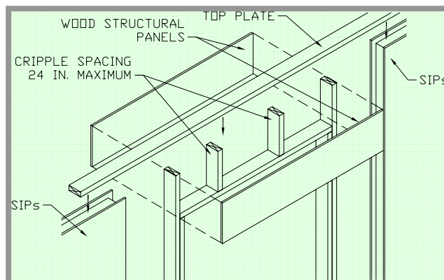
Figure 5.1 Typical Wood Structural Panel Box Header Construction
