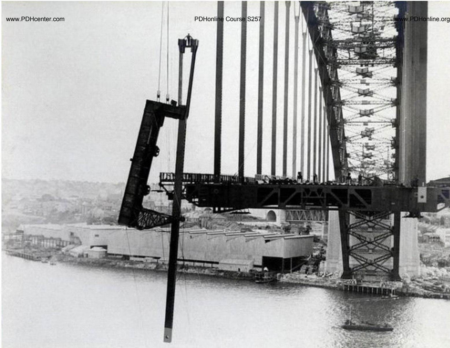
Hanger being lifted in special cradle
