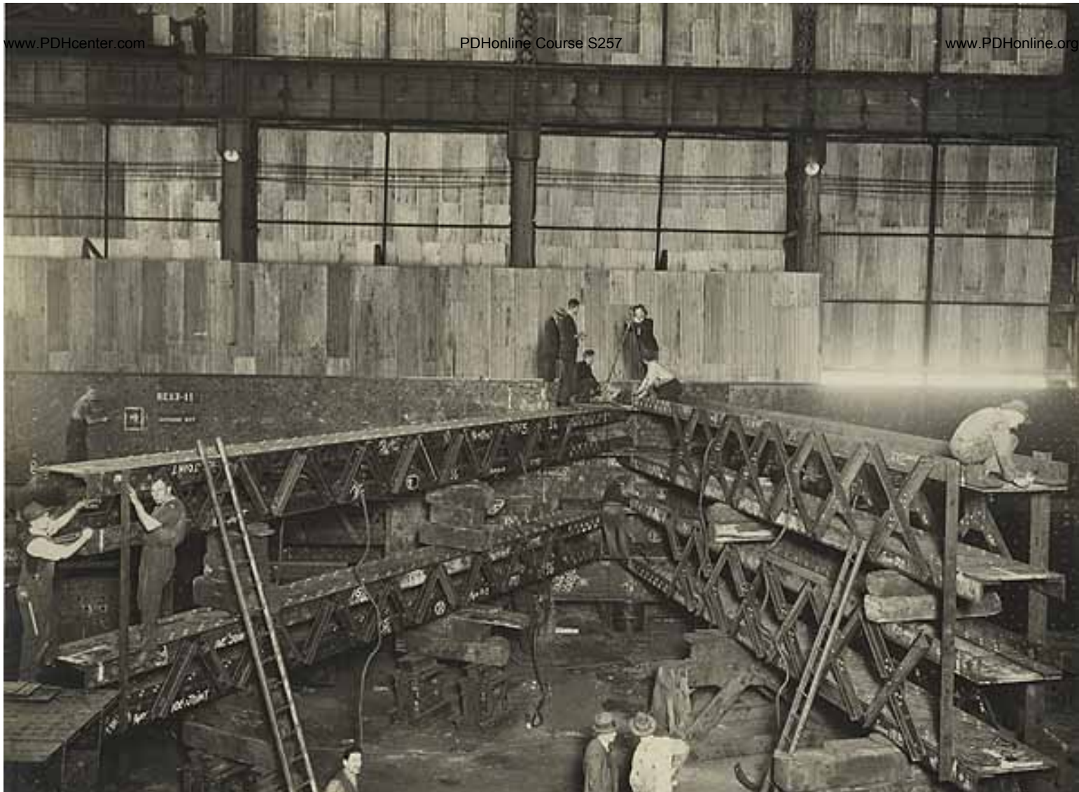
Assembly of “Joint 13” - April 15, 1930 (Heavy Workshop)
