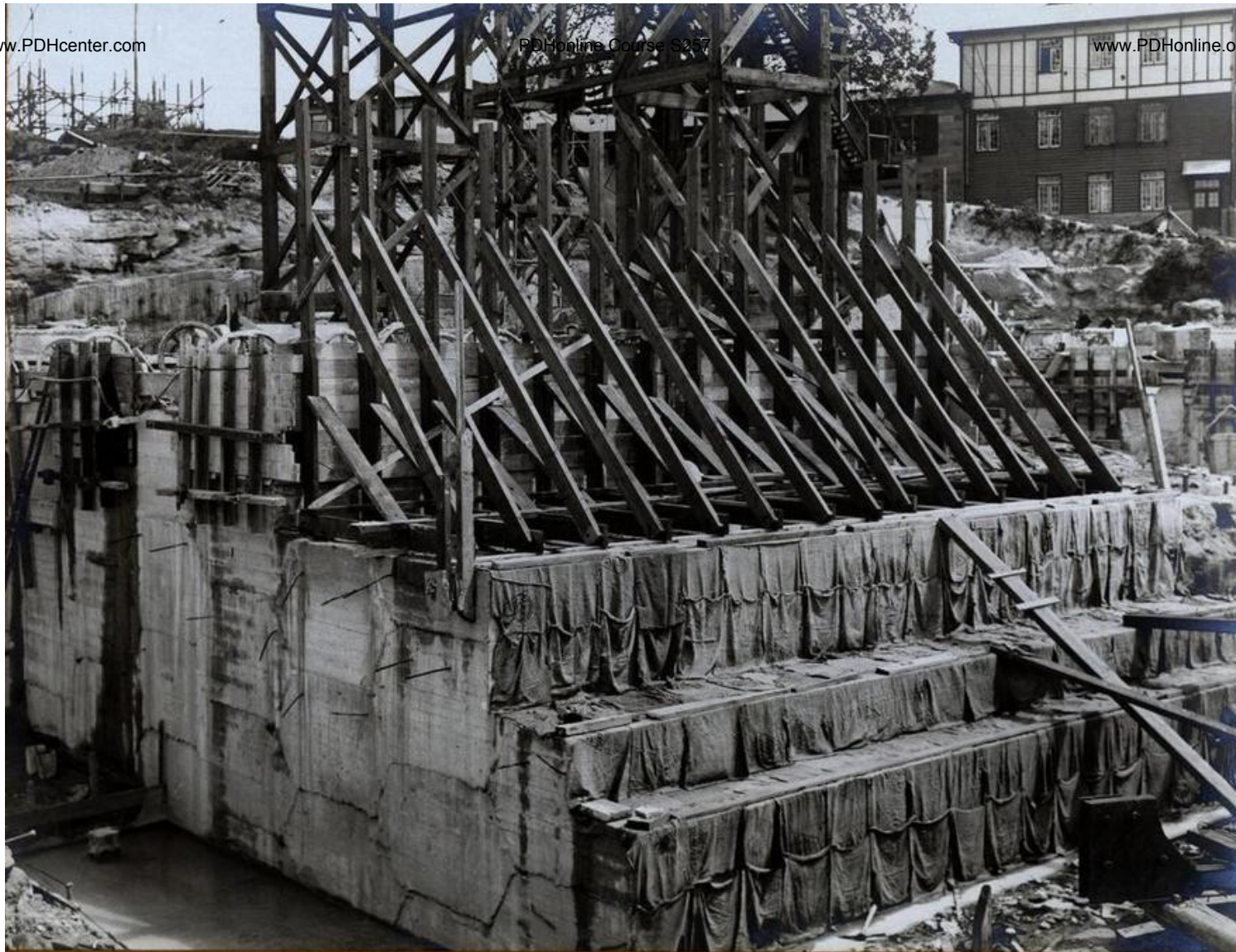
Skewback concrete stepped to receive special concrete (under main hinge-bearing)
