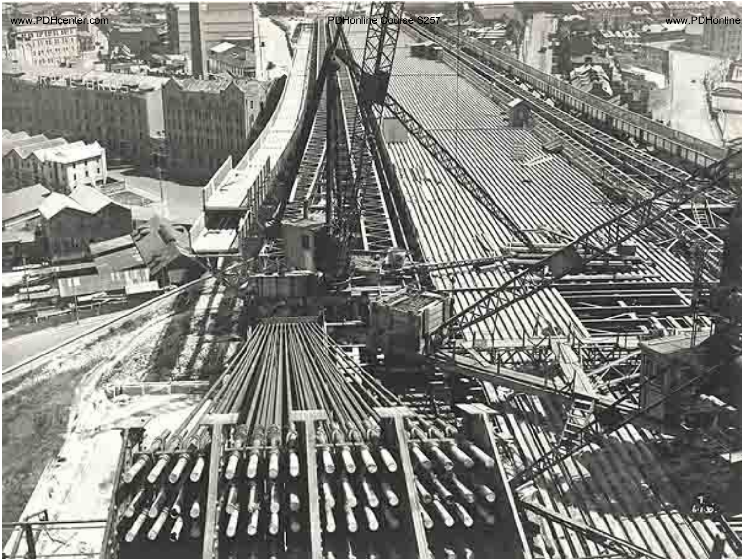
Looking down at wire cable “Container” (from atop upper chord)
