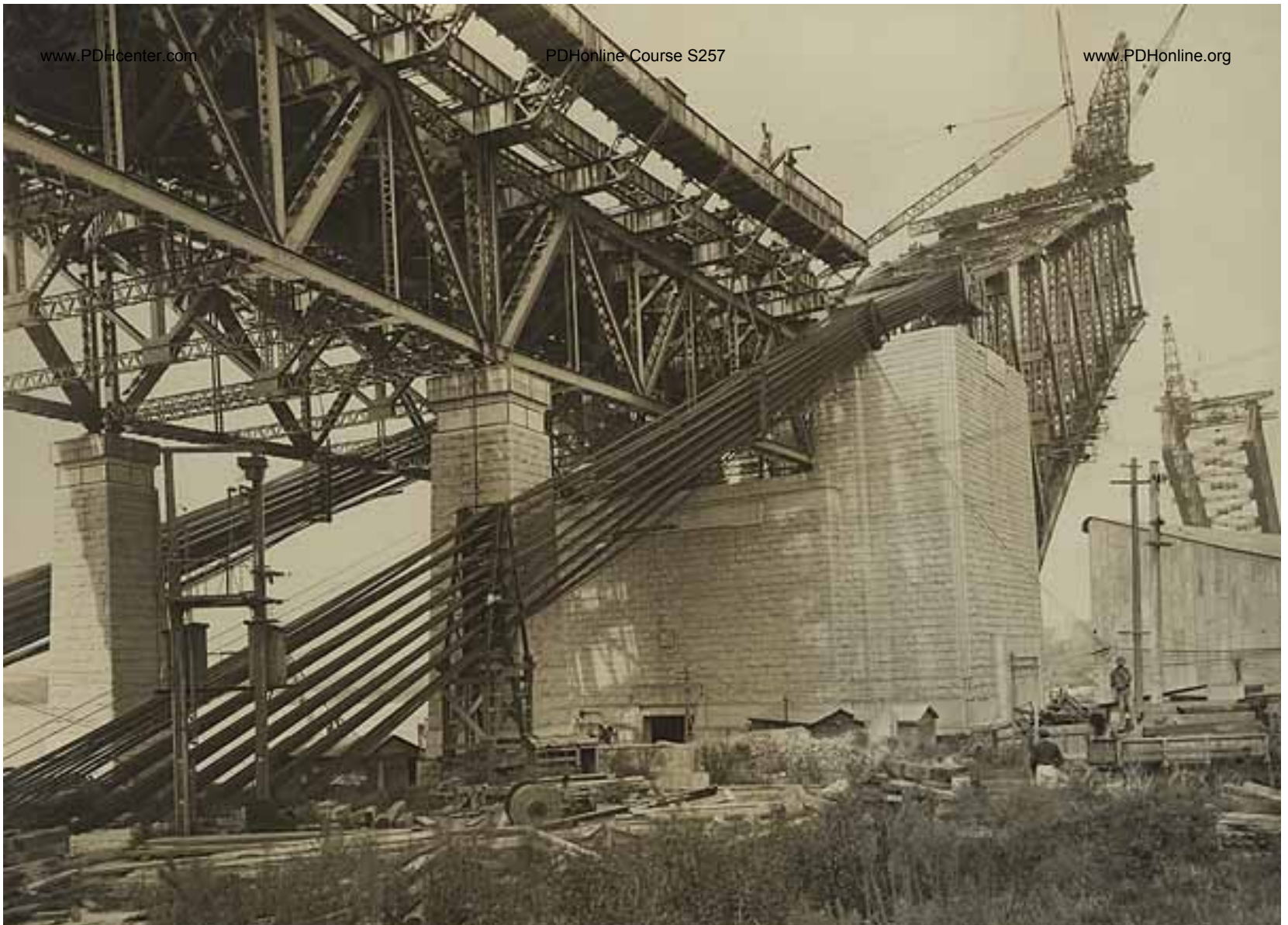
Alignment/support tower (before entering tunnel)
