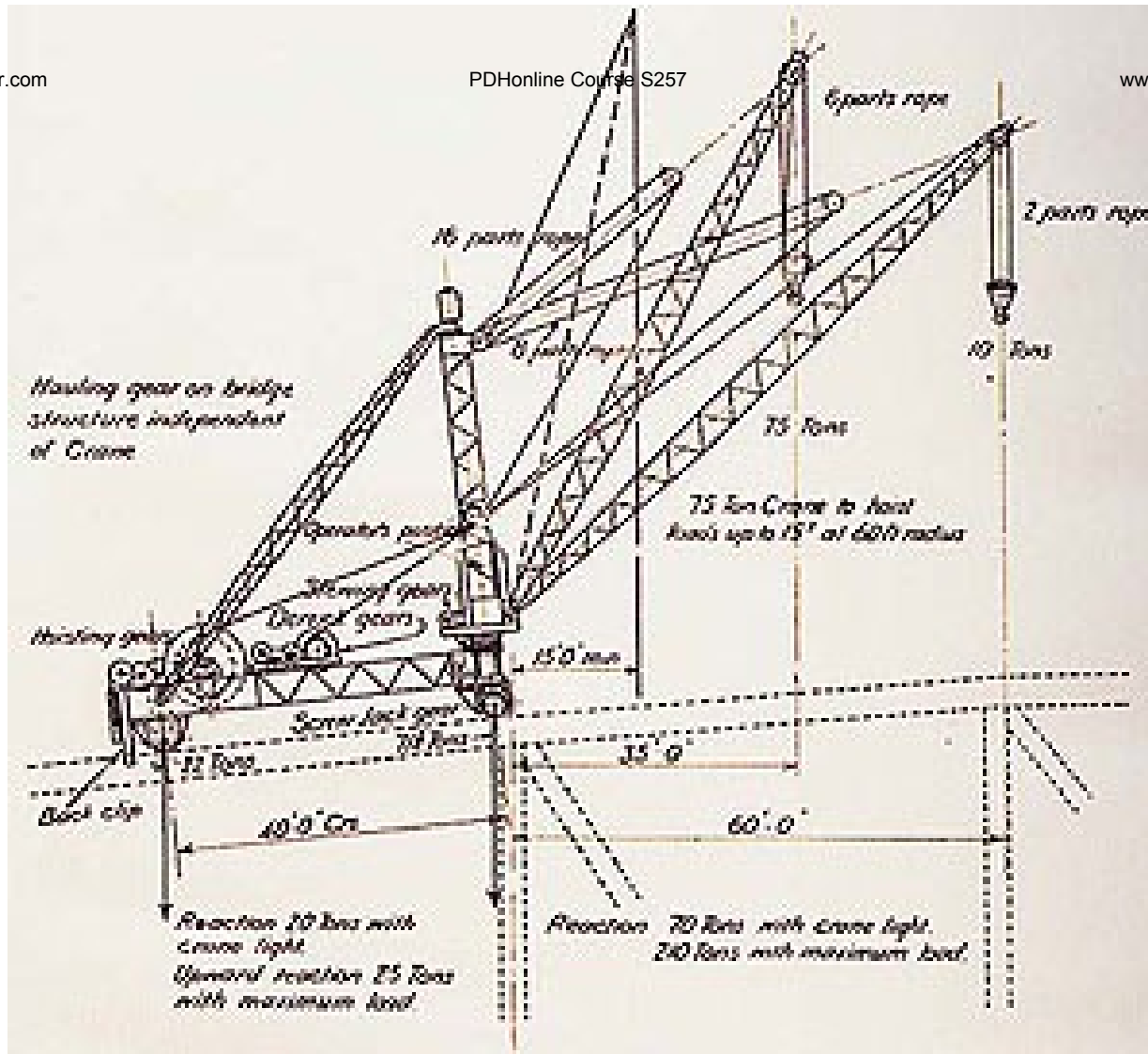
Diagram of a Crawler Crane from Sydney Harbour Bridge: Report on Tenders (hauling gear on bridge structure independent of (main) crane)
