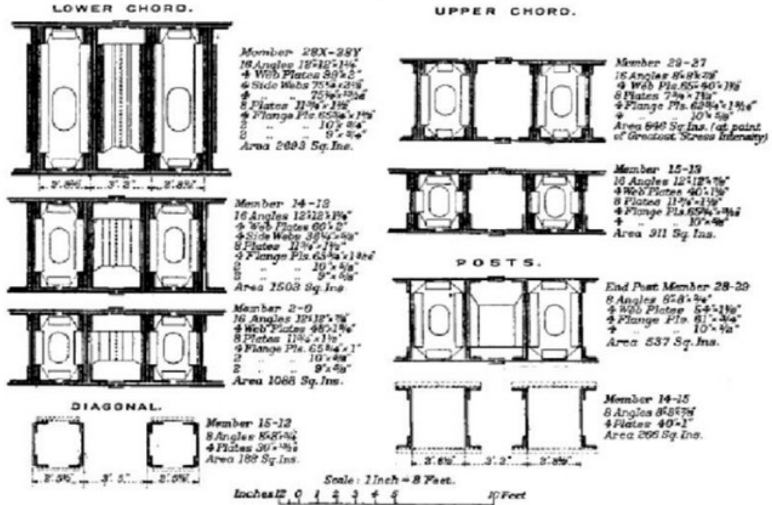
TYPICAL CROSS SECTIONS OF MEMBERS.
