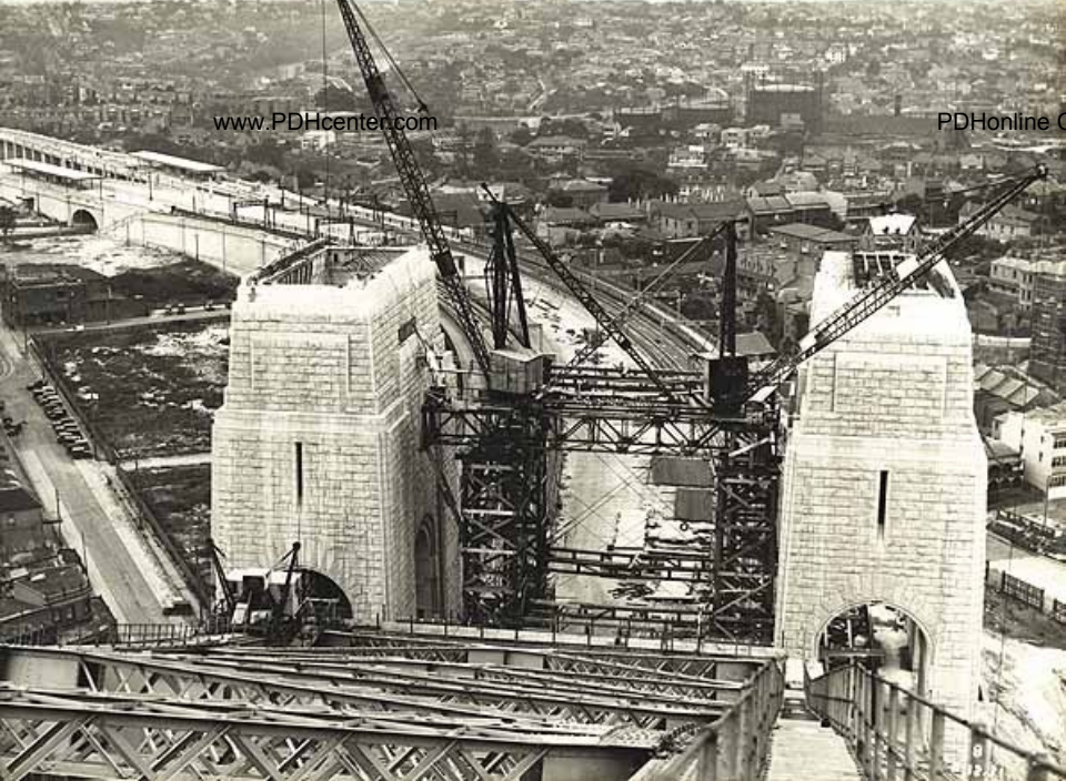
N. Pylon (top left) and S. Pylon (top right) nearing completion
