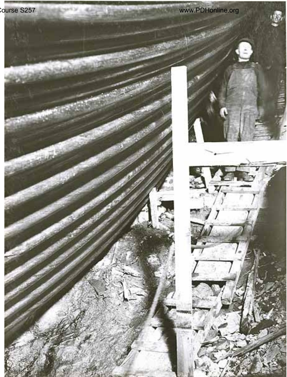
Wire cables passing around inner tunnel wall 192
