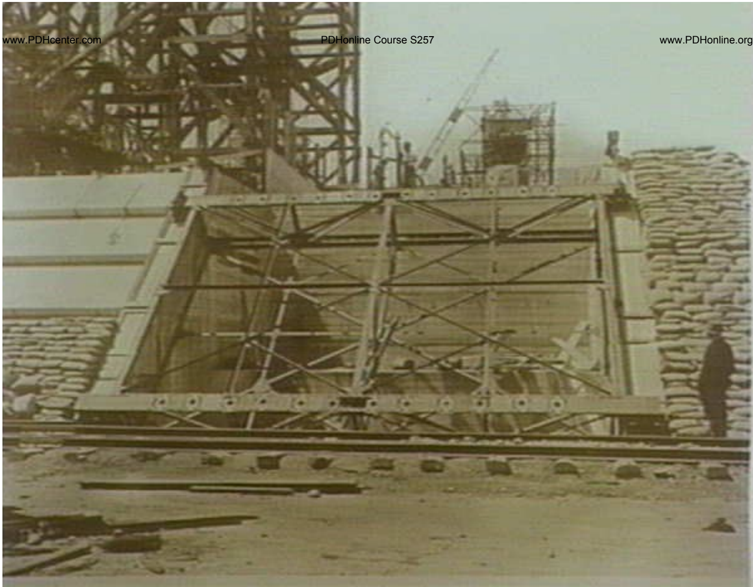
Temporary steel frame over Skewback (to support hinge-bearing during adjustment) 168
