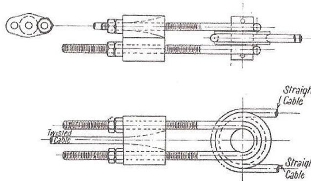
DETAIL OF SHACKLES
