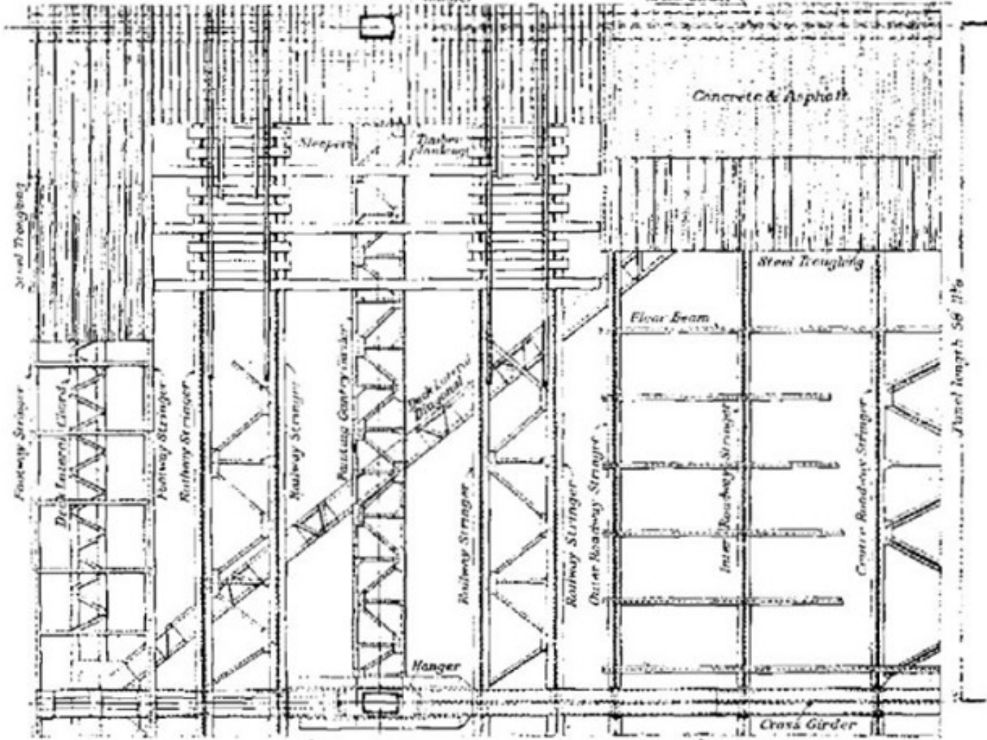
Half-plan of one panel of deck
