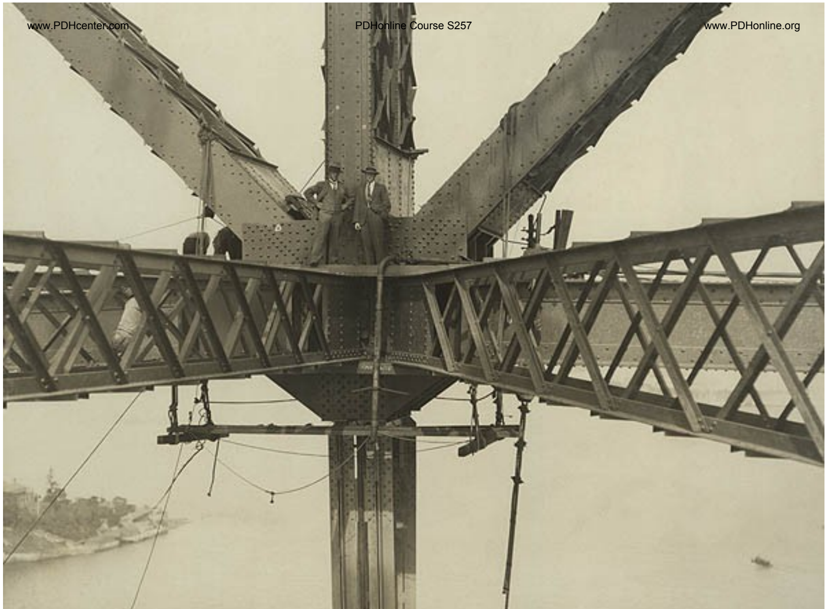
Center hanger secured to panel point in lower chord 328
