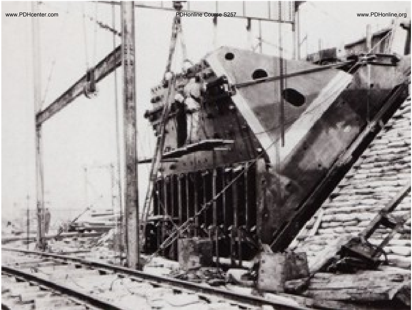
Pedestal (a.k.a. “Saddle”) secured in place (atop Base)
