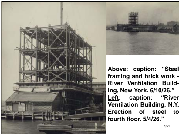
Above: caption: "Steel framing and brick work - River Ventilation Building, New York. 6/10/26." Left: caption: "River Ventilation Building, N.Y. Erection of steel to fourth floor. 5/4/26." 551
