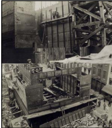
Top: caption: "General view, West side, tube opening. Showing riveters at work, lines of air hose. Spring Street, May 6, 1921" Bottom: caption: "General view, East side. Subway opening. Spring Street, May 6, 1921"
