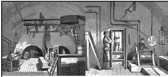
Left: caption: "View inside the caisson looking east toward the twin tubes. The larger air lock is on the right, and the smaller one for materials is in the center background. From Scientific American , June 4, 1881)"
