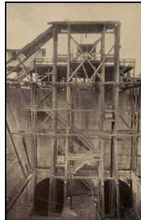
Left: caption: "Weehawken Shaft, 100x154 ft. at top; 56x116 ft. at bottom; 76 ft. deep; lined with 9,810 cu. ft. concrete; begun June 11, 1903, finished Sept. 1, 1904. Manhattan Shaft, 22x32 ft.; 55 ft. deep; begun June 10, 1903; finished Dec. 11. Built by United Eng. & Con. Co."
