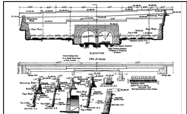
Above: caption: "Portal, Retaining and Face Walls, Tenth Avenue." Drains were left behind the portal around the back of each arch, leading down to the bottom and through the concrete base at each side of the portal and in the central core-wall.
