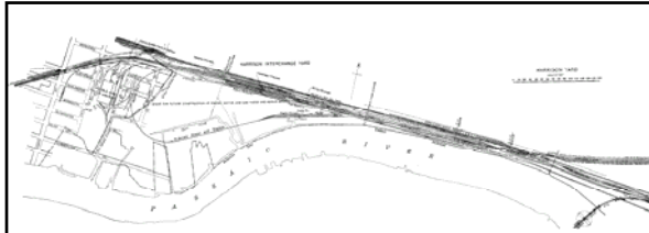
Above: caption: "Plan of Harrison Yard." West of the Hackensack portal, the Meadows Division project included five miles of double-track line on a high fill across the Hackensack Meadows to a junction with the PaRR's New York Division main line at Harrison. Work included: • A drawbridge at a crossing of the Hackensack River • Yard and terminal facilities at Harrison (where the change between steam and electric motive power would take place) • A new station named Manhattan Transfer (where passengers could transfer between trains on the PaRR lines to Manhattan and/or Jersey City and the H&MRR)" 259
