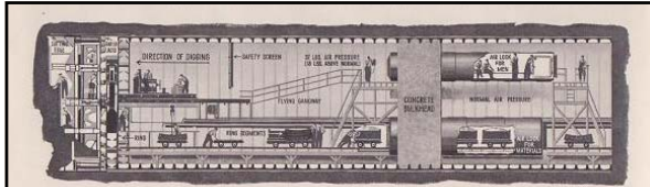
"...The diagram above shows how a tunnel is bored through rock and silt. Because work is carried on 20 ft. under the river bed, the sandhogs wage a continual battle to keep water from pouring into the tunnel. Only practical way of keeping it out is to use compressed air. Hence a massive concrete bulkhead is built near each end of the tube. Men passing through the bulkhead enter air locks in which air pressure is gradually raised to that prevailing on other side. At left is the working end of the shaft composed of a big circular shield and a row of hydraulic jacks. As the shield is jacked forward, silt is displaced and some is forced through shield apertures. After each shove a cast-iron ring forming outer jacket of the tunnel is brought in in segments and placed in position. Bull's eye of the two shields pushing from each end of the tube was a big steel caisson sunk in the New York edge of the Hudson River bed. When the shield reached this caisson they burned through its steel walls and the tunnel was holed through..." 805 LIFE magazine, December 27 th 1937
