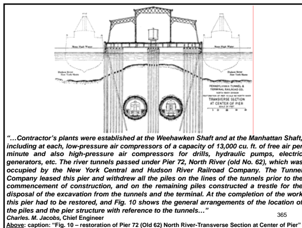
Above: caption: "Fig. 10 - restoration of Pier 72 (Old 62) North River-Transverse Section at Center of Pier"
