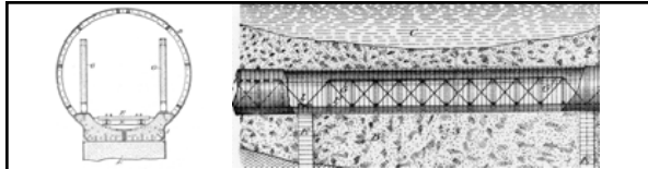
Above: caption: “These Patent Office drawings, reproduced from the February 11, 1902, issue of Scientific American, show the ‘tunnel bridge’ scheme devised by Charles M. Jacobs to support a tunnel driven through silt or other loose material. The track was to be carried by steel trusses, which were to be surrounded by the tunnel shell and supported by piers sunk through the river bottom silt to rock or other firm material.” An early problem was that of assuring adequate stability of the tubes in the soft silt of the riverbed under heavy loads. In 1901, Chief Engineer Charles Jacobs proposed and, in 1902, patented a “subterranean tunnel bridge” design for the crossing consisting of piers carried to a solid foundation in the riverbed, a truss bridge carried on the piers and a tunnel shell surrounding the bridge and attached to the piers. The bridge structure would carry the live load of trains directly to the piers, avoiding any deflection of the tunnel. The v-truss bridge scheme was soon discarded in favor of one that called for the use of shorter girders that would support the track and the trains. They would be carried on piers spaced at 15-foot intervals. The method was tested near the New Jersey bank of the river.
