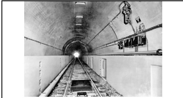
Above: caption: "The completed tunnel looked like this. The concrete 'benches' on either side of the track were designed to confine a train to the center of the track in case of a derailment, and provided, at the right, a walkway for the placement of signals and a place for signal maintainers to work safely, and, at the left, a safe exit from the tunnel. The 675-volt DC third rail is at the left of the track. The photograph was taken in the westbound tunnel, facing towards the Weehawken shaft." 397
