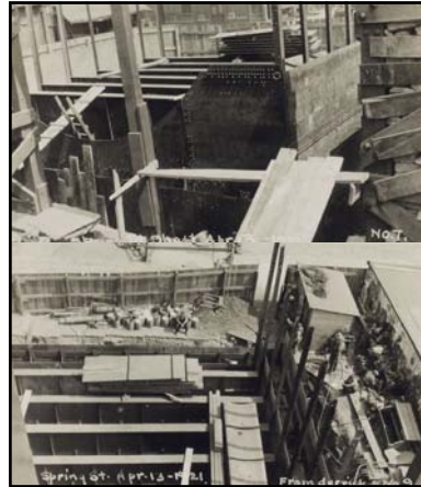
Top: caption: "Roof girders of working chamber in place. Spring Street shaft, April 13, 1921" Bottom: caption: "Roof girders and sided angles, roof plates on blocking. Spring Street, April 13, 1921"
