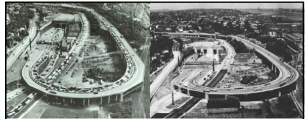
Left: caption: "New Jersey Plaza and Helix prior to start of construction of the Third Tube Project" Right: caption: "New Jersey Plaza and Helix after completion of the Third Tube Project. Note third portal, new administration building, widened tolls area, new center ramp, widened westbound helix." 934
