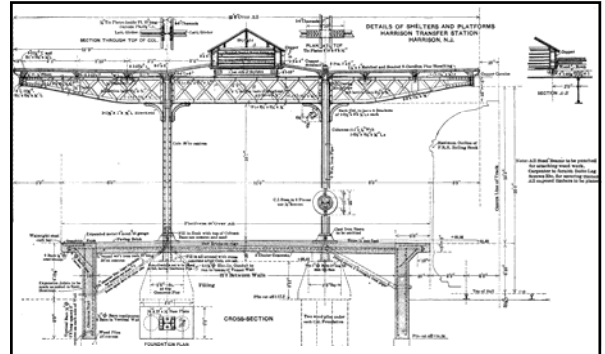
Above: caption: "Details of Shelters and Platforms Harrison Transfer Station Harrison, N.J." 260
