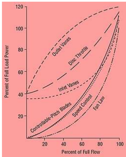
Fan and system curves to show the effects of different flow controls
