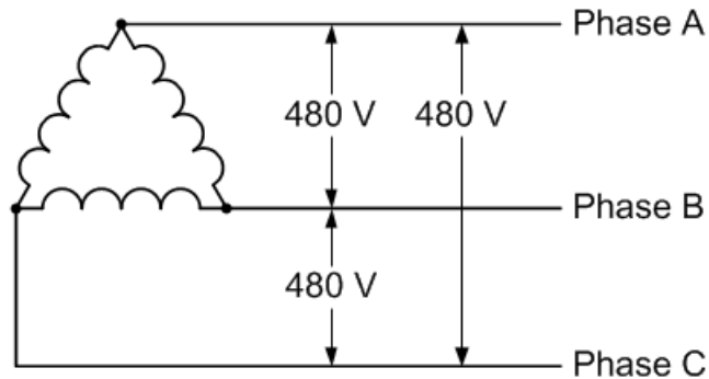
Three Phase Three Wire Delta
