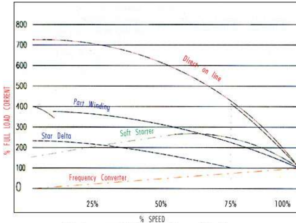
Starting current of various types of starters
