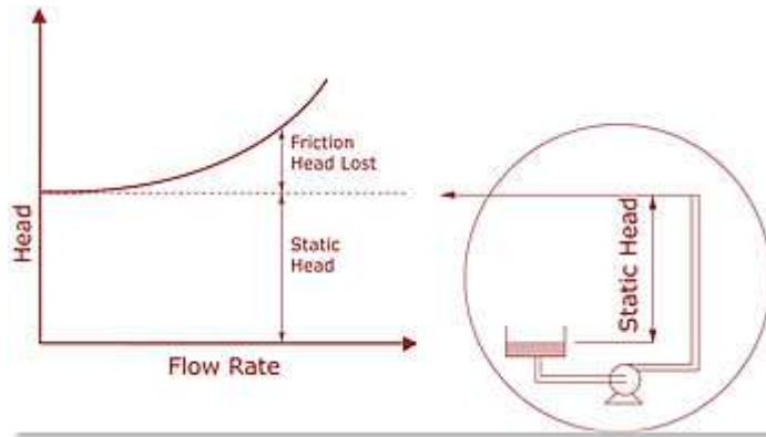
System curve showing static head and friction head lost
