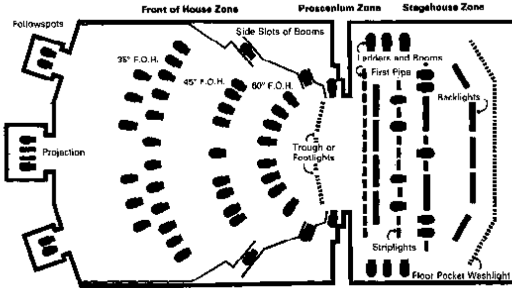
Diagrammatic Plan
