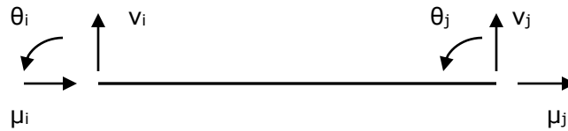
Figure 4 – Degrees-of-Freedom of a Typical 2-D Beam Element
